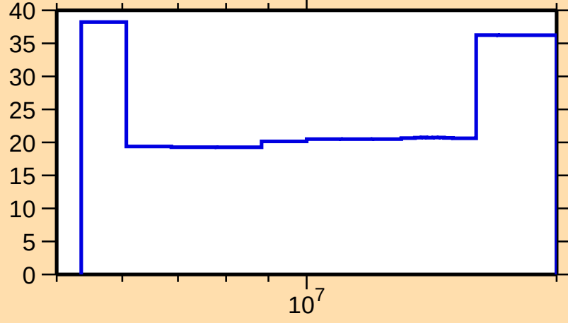
\Delta\sigma/\sigma vs. E for ^{132}\text{Sb}(n,2n)
