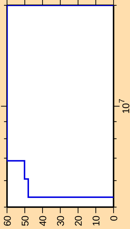
\Delta\sigma/\sigma vs. E for ^{132}\text{Sb}(n,n_1)
