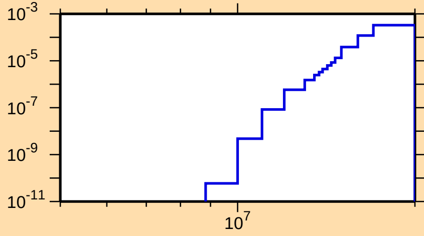
\sigma vs. E for ^{132}\text{Sb}(n,t)
