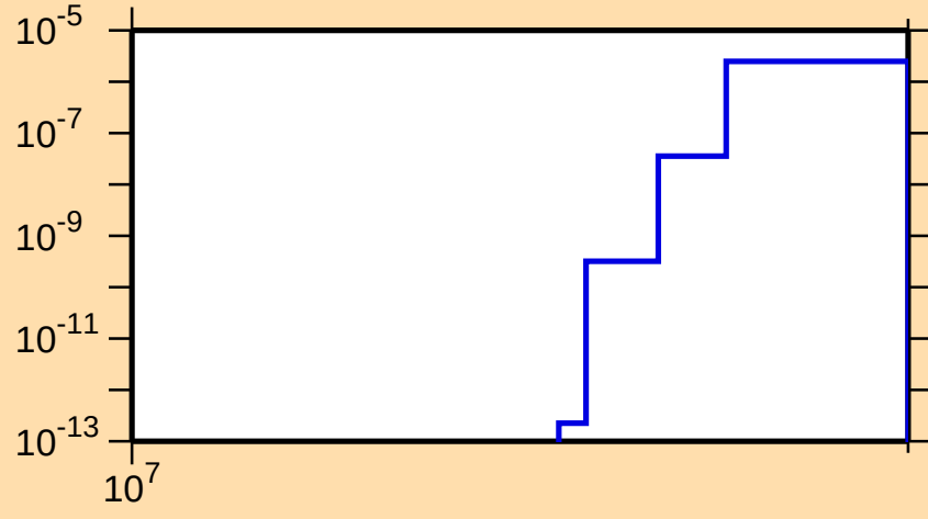
\sigma vs. E for ^{132}\text{Sb}(n,\text{nd})
