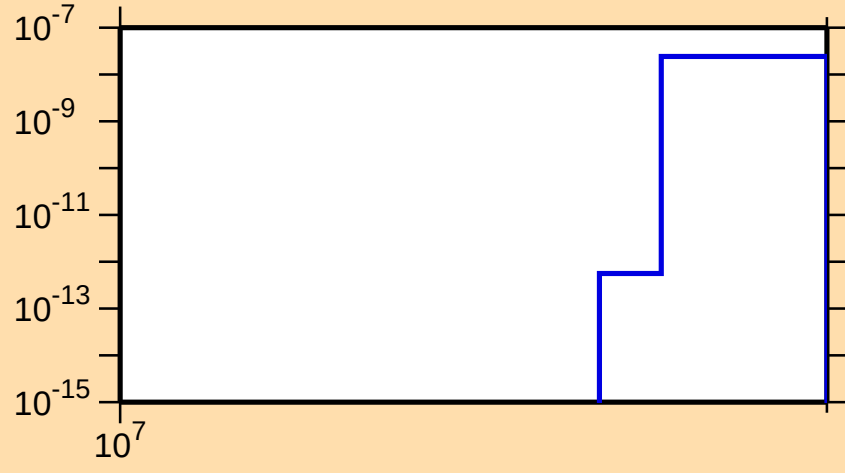
\sigma vs. E for ^{132}\text{Sb}(n,2np)
