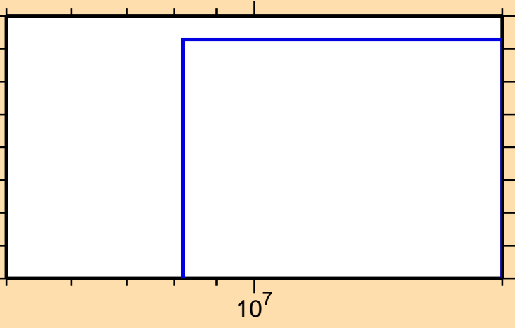
\sigma vs. E for ^{132}\text{Sb}(n,t)
