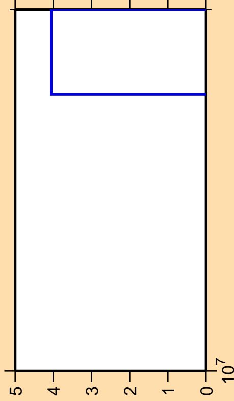
\Delta\sigma/\sigma vs. E for ^{44}\text{Sc} (mt 34)
