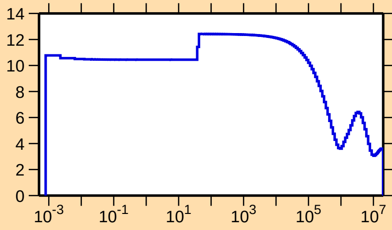
\sigma vs. E for ^{273}
