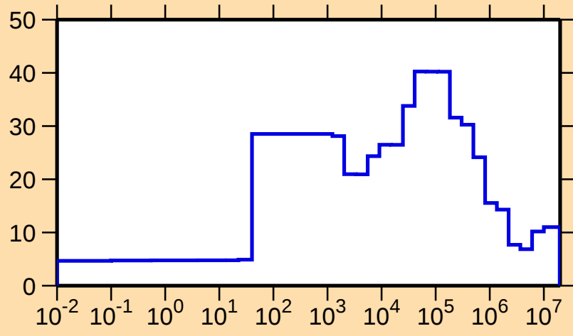
\Delta\sigma/\sigma vs. E for ^{273}\text{Ge}
