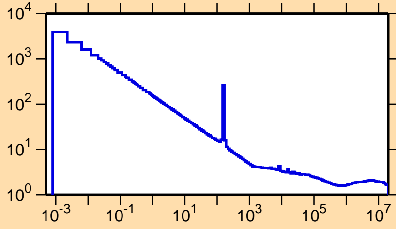
\sigma vs. E for ^{102}\text{Sn}(n,\text{nonel.})
