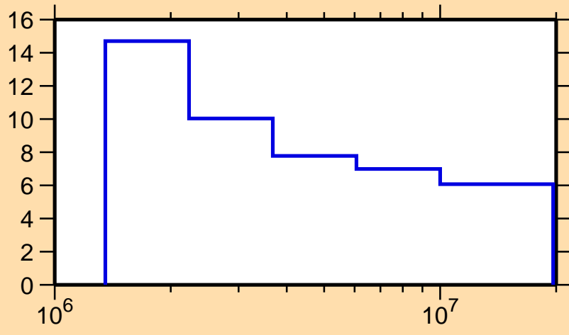
\Delta\sigma/\sigma vs. E for ^{102}\text{Sn}(n,\text{nonel.})
