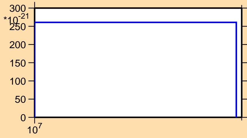
\sigma vs. E for ^{102}\text{Sn}(n,nt)
