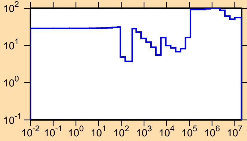
\Delta\sigma/\sigma vs. E for ^{102}\text{Sn}(n,\gamma)
