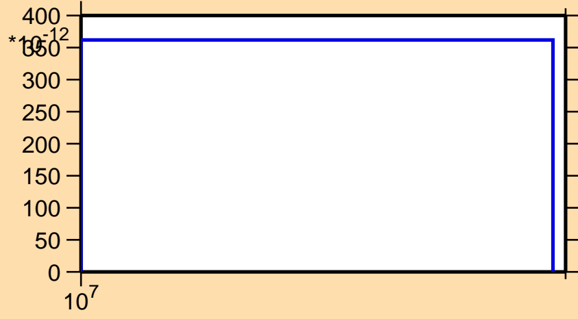
\sigma vs. E for ^{102}\text{Sn}(n,\text{nd})
