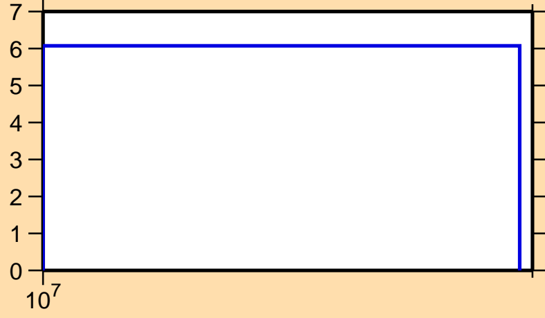
\Delta\sigma/\sigma vs. E for ^{102}\text{Sn}(n,\text{nonel.})
