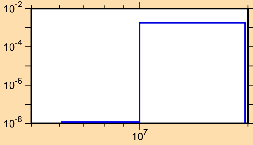
\sigma vs. E for ^{102}\text{Sn}(n,\text{pd})
