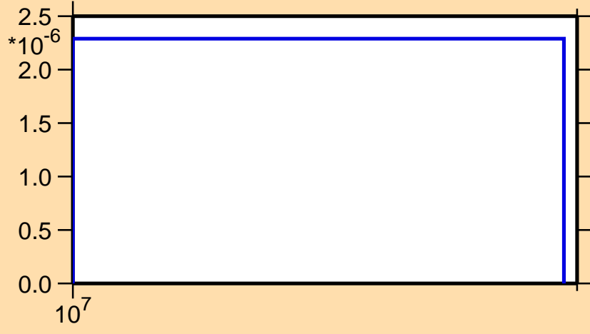
\sigma vs. E for ^{102}\text{Sn}(n,\text{pt})
