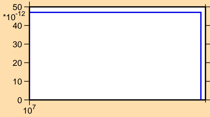
\sigma vs. E for ^{102}\text{Sn} (mt 34)
