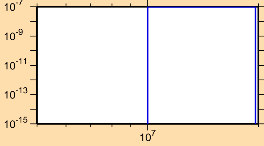
\sigma vs. E for ^{102}\text{Sn}(\text{mt } 45)
