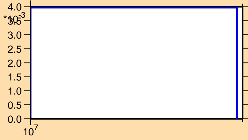
\sigma vs. E for ^{102}\text{Sn}(n,2n)
