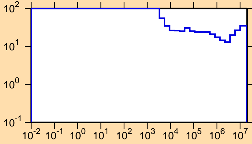
\Delta\sigma/\sigma vs. E for ^{102}\text{Sn}(n,p)
