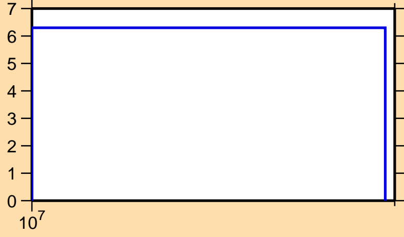
\Delta\sigma/\sigma vs. E for ^{102}\text{Sn}(n,\text{tot.})
