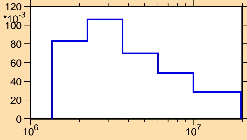
\sigma vs. E for ^{102}\text{Sn}(n,n_1)
