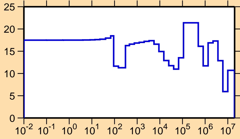
\Delta\sigma/\sigma vs. E for ^{102}\text{Sn}(n,\text{el.})
