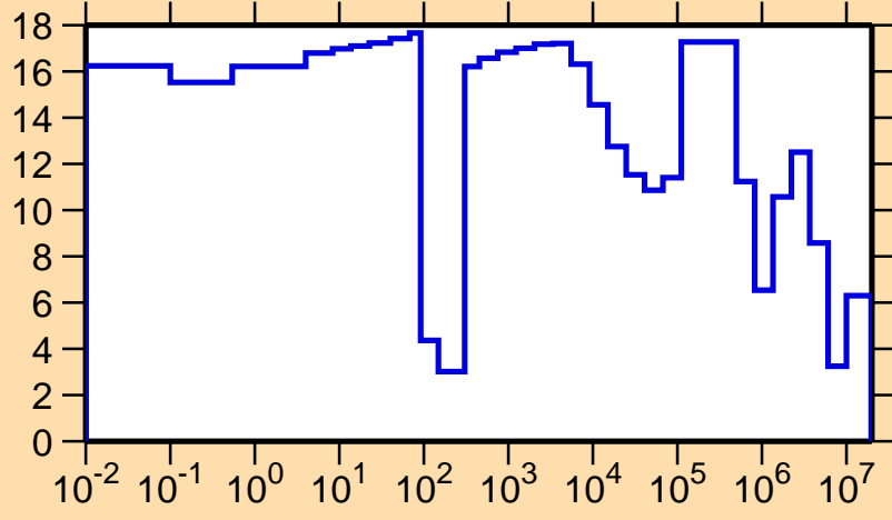
\Delta\sigma/\sigma vs. E for ^{102}\text{Sn}(n,\text{tot.})
