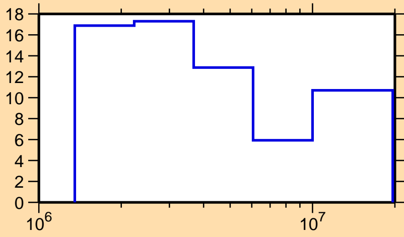
\Delta\sigma/\sigma vs. E for ^{102}\text{Sn}(n,\text{el.})
