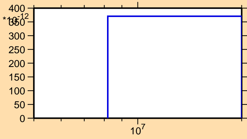
\sigma vs. E for ^{102}\text{Sn}(n,\text{nd})
