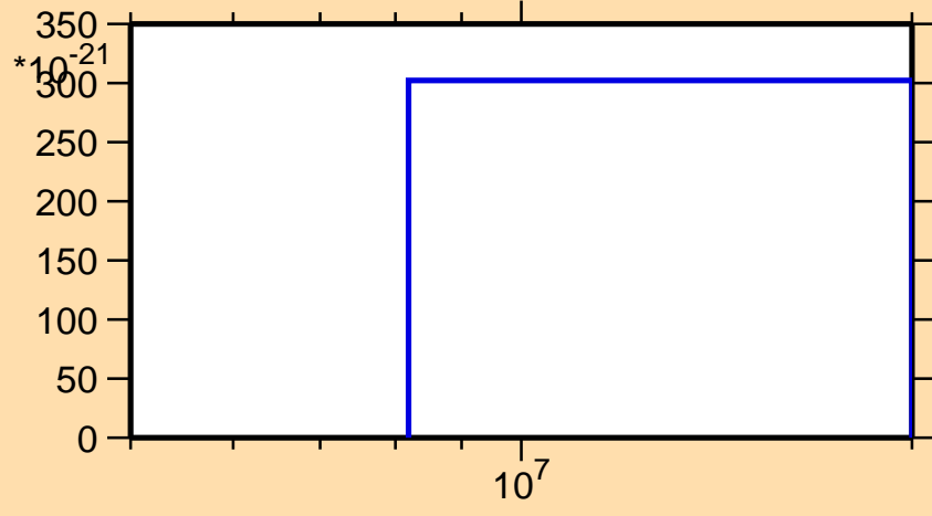
\sigma vs. E for ^{102}\text{Sn}(n,nt)
