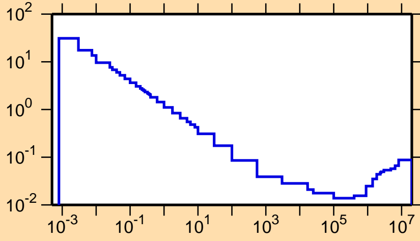
\sigma vs. E for ^{102}\text{Sn}(n,\alpha)
