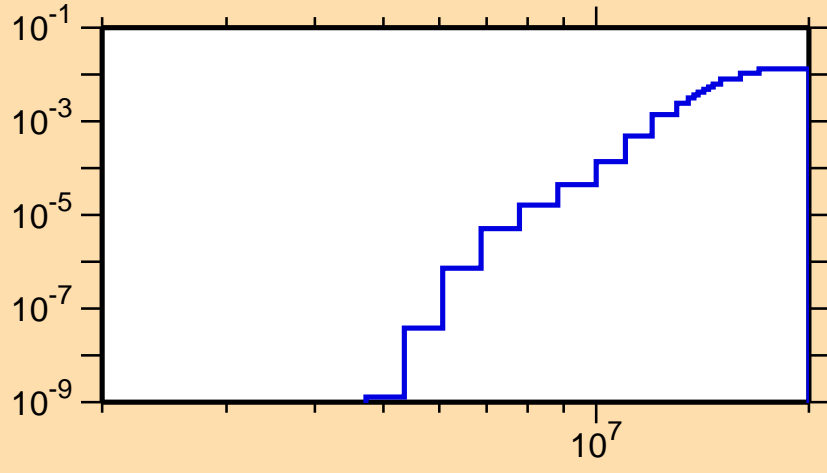
\sigma vs. E for ^{103}\text{Sn}(n,n\alpha)
