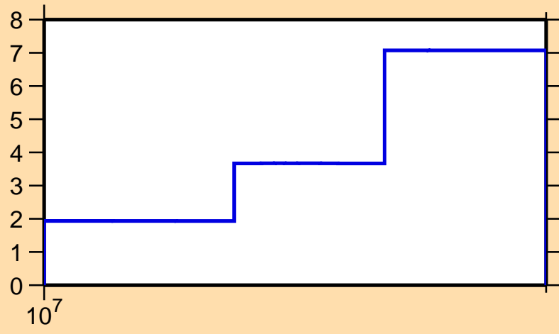
\Delta\sigma/\sigma vs. E for ^{103}\text{Sn}(n,\text{tot.})
