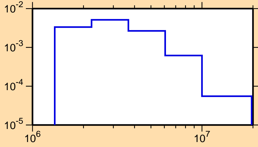
\sigma vs. E for ^{103}\text{Sn}(n,n_3)
