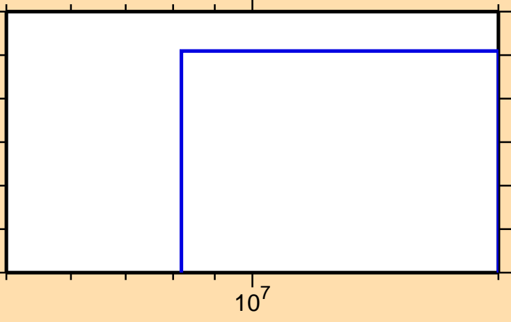
\sigma vs. E for ^{103}\text{Sn}(n,\text{pt})
