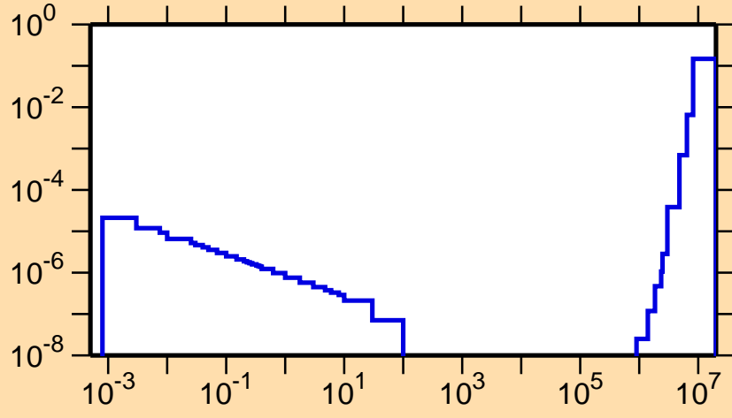
\sigma vs. E for ^{103}\text{Sn}(n,p\alpha)
