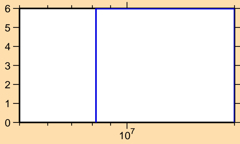
\Delta\sigma/\sigma vs. E for ^{103}\text{Sn}(n,\text{nonel.})
