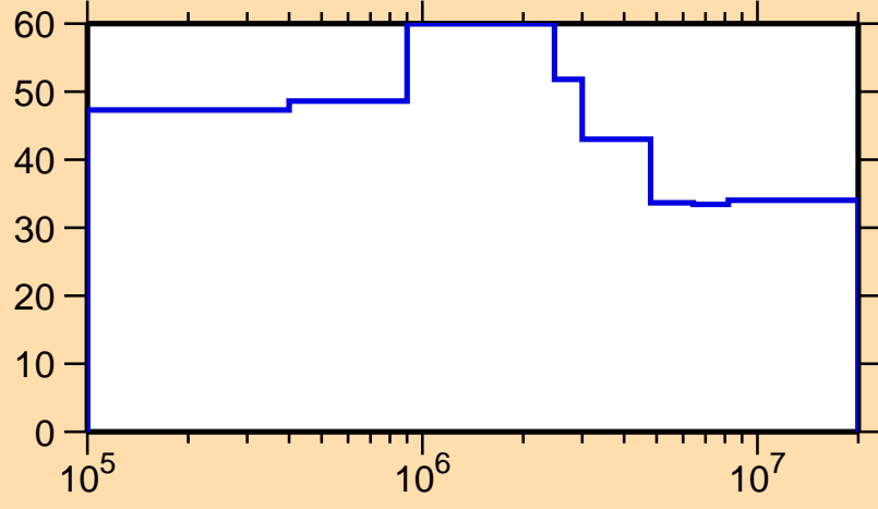
\Delta\sigma/\sigma vs. E for ^{103}\text{Sn}(n,n_1)
