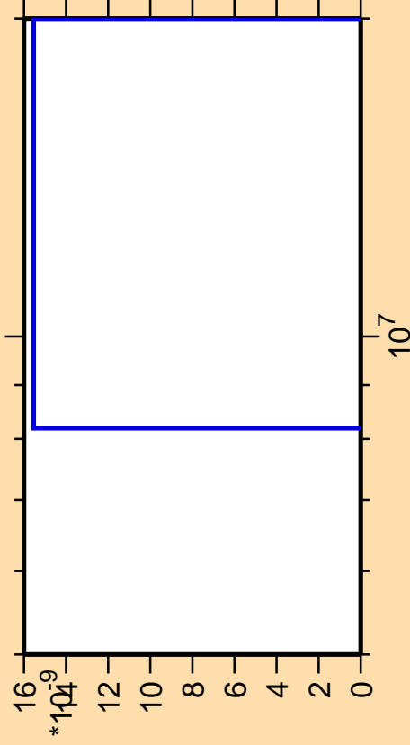
\Delta\sigma/\sigma vs. E for ^{103}\text{Sn}(n,nt)
