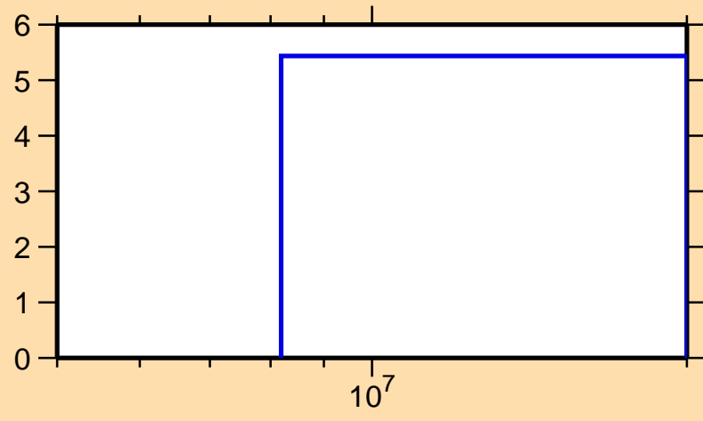
\Delta\sigma/\sigma vs. E for ^{103}\text{Sn}(n,\text{el.})
