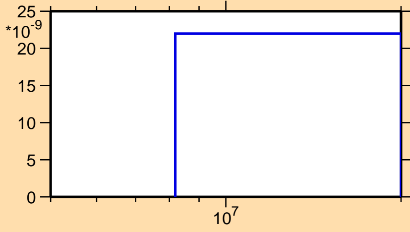
\sigma vs. E for ^{103}\text{Sn}(\text{mt117})
