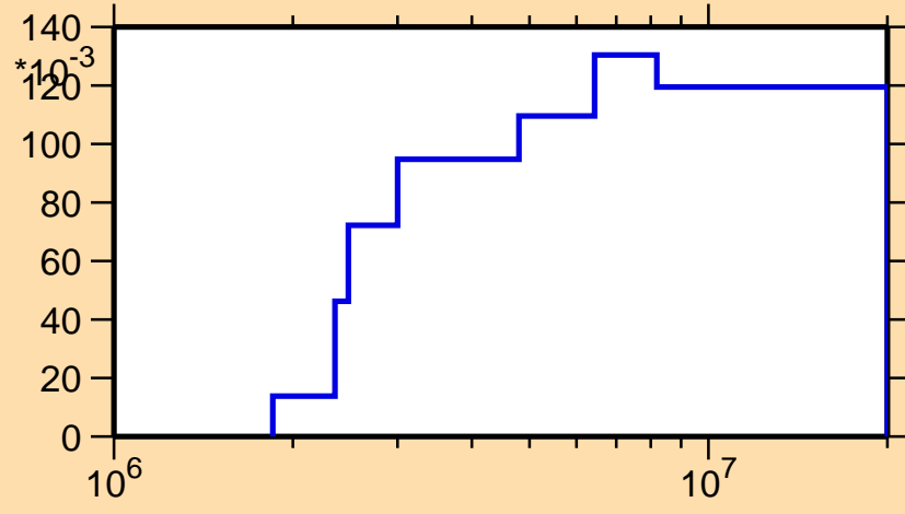
\sigma vs. E for ^{103}\text{Sn}(n,n\text{cont.})
