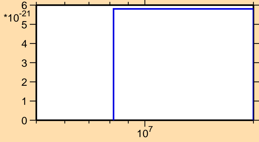
\sigma vs. E for ^{103}\text{Sn}(n,nt)
