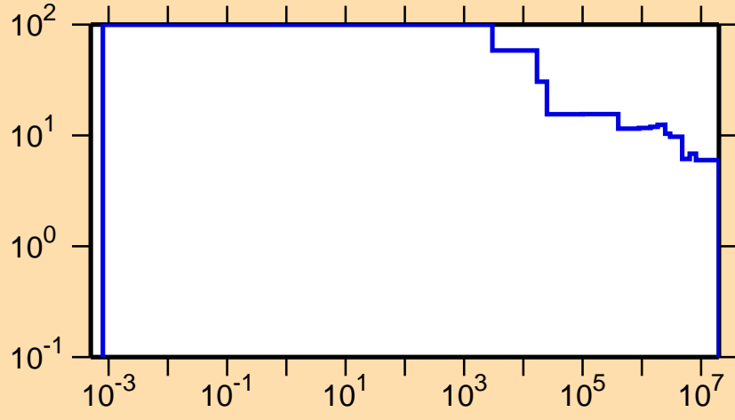
\Delta\sigma/\sigma vs. E for ^{103}\text{Sn}(n,\text{nonel.})
