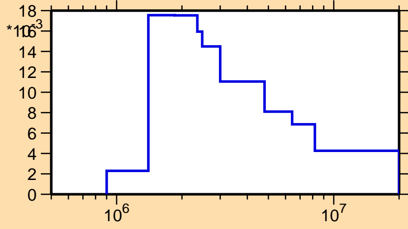
\sigma vs. E for ^{103}\text{Sn}(n,n_2)
