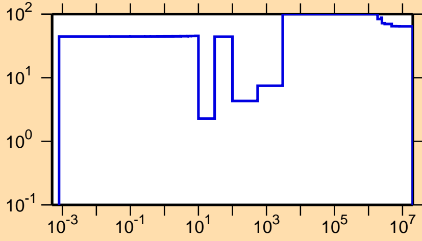
\Delta\sigma/\sigma vs. E for ^{103}\text{Sn}(n,\gamma)
