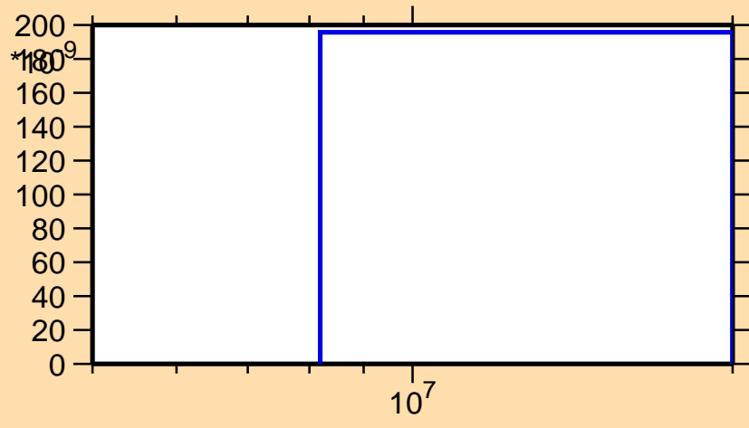
\sigma vs. E for ^{103}\text{Sn}(n,2np)
