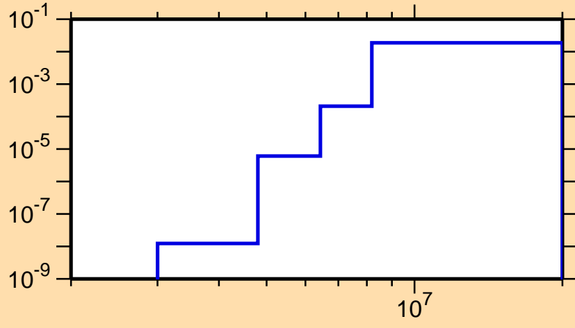
\sigma vs. E for ^{103}\text{Sn}(n,d)
