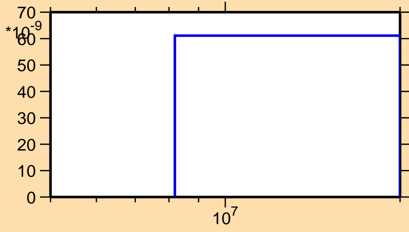
\sigma vs. E for ^{103}\text{Sn}(n,\text{nd})
