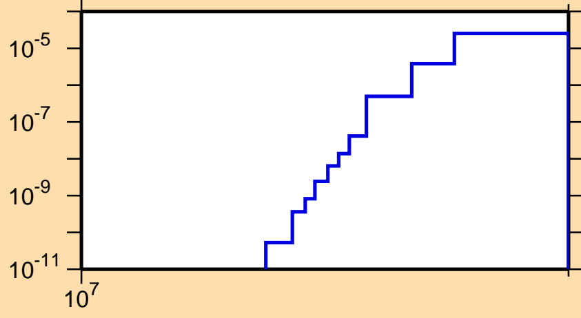
\sigma vs. E for ^{109}\text{Sn}(n,\text{pd})
