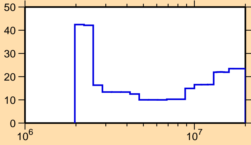
\Delta\sigma/\sigma vs. E for ^{109}\text{Sn}(n,n\text{cont.})
