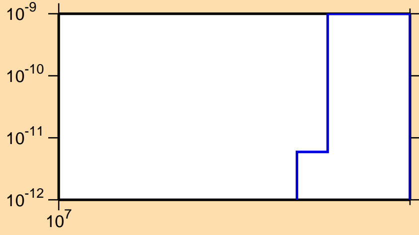
\sigma vs. E for ^{109}\text{Sn}(\text{mt } 34)
