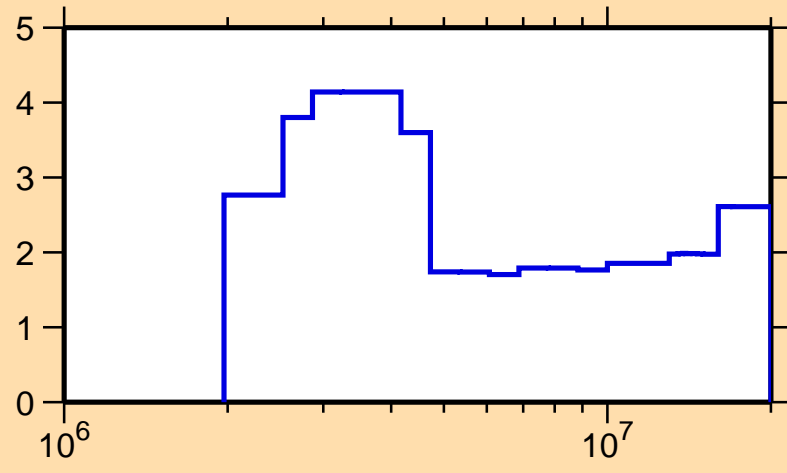
\Delta\sigma/\sigma vs. E for ^{109}\text{Sn}(n,\text{tot.})
