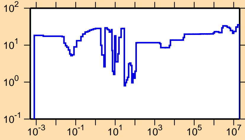
\Delta\sigma/\sigma vs. E for ^{109}\text{Sn}(n,\gamma)
