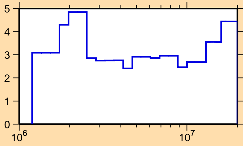
\Delta\sigma/\sigma vs. E for ^{110}\text{Sn}(n,\text{el.})
