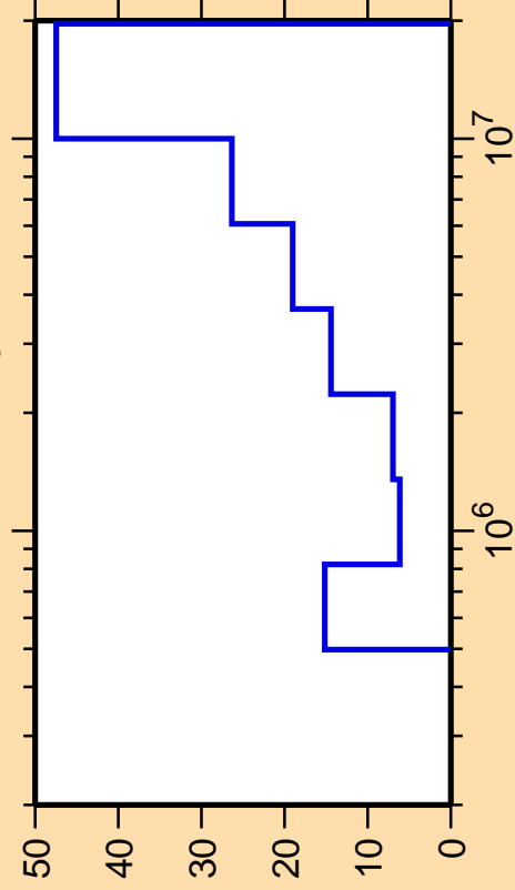
\Delta\sigma/\sigma vs. E for ^{113}\text{Sn}(n,n_3)
