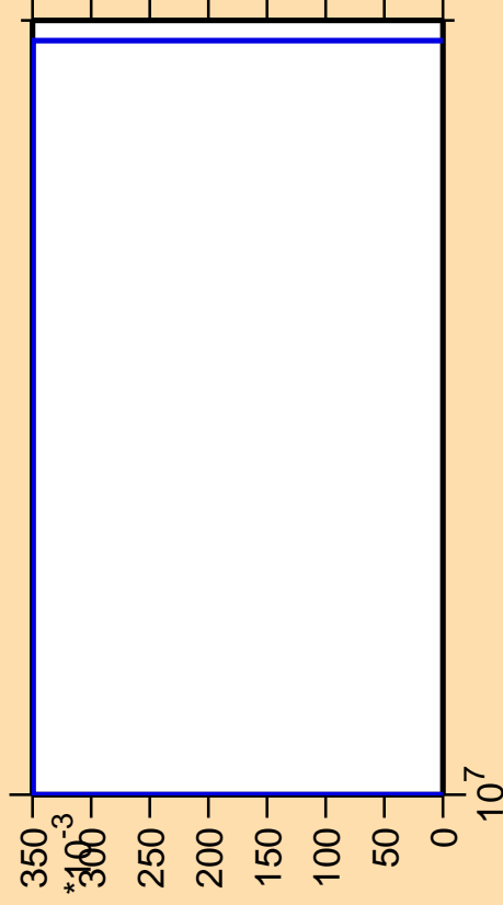
\Delta\sigma/\sigma vs. E for ^{113}\text{Sn}(n,\text{pt})
