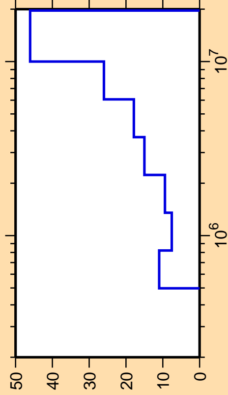
\Delta\sigma/\sigma vs. E for ^{113}\text{Sn}(n,n_4)
