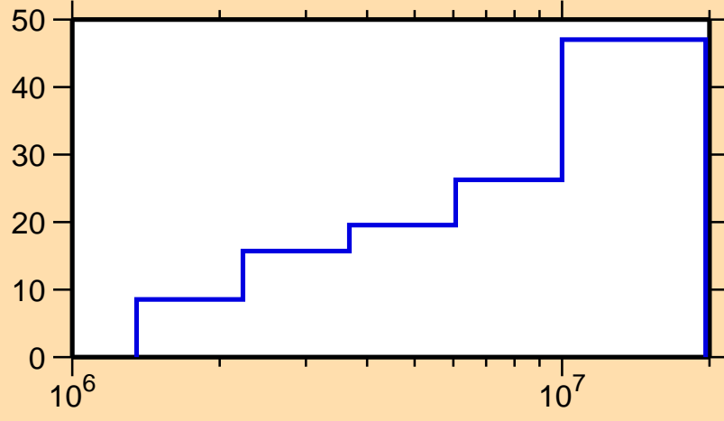
\Delta\sigma/\sigma vs. E for ^{113}\text{Sn}(n, n_1)
