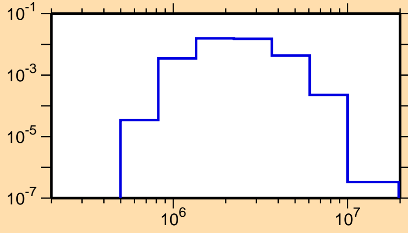
\sigma vs. E for ^{113}\text{Sn}(n,n_4)
