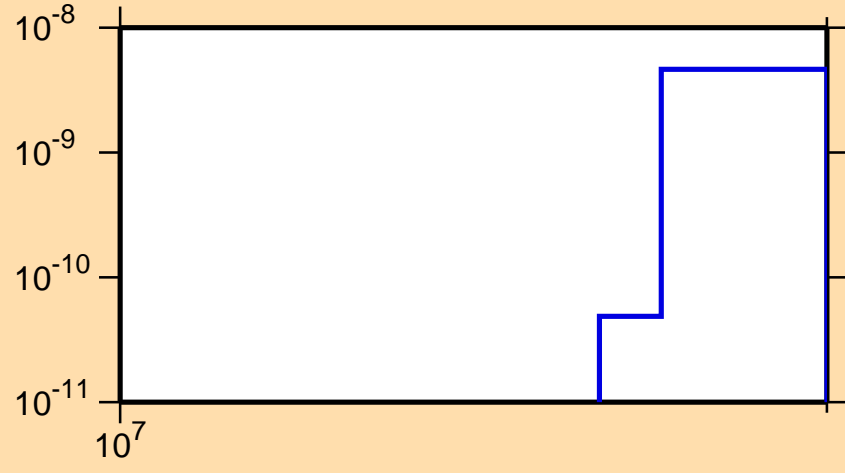
\sigma vs. E for ^{116}\text{Sn}(n,\text{He}3)
