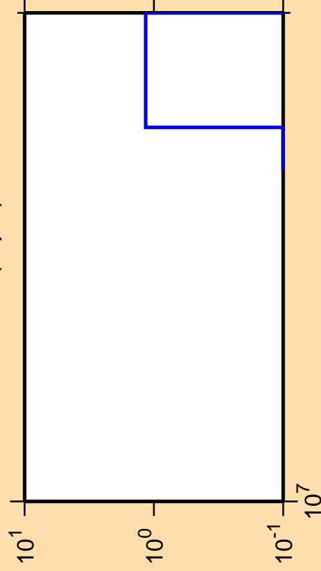
\Delta\sigma/\sigma vs. E for ^{116}\text{Sn}(n,p\alpha)
