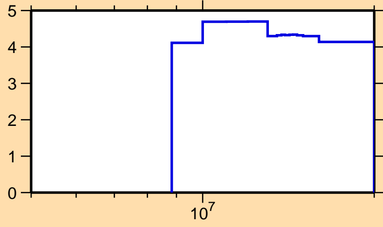
\Delta\sigma/\sigma vs. E for ^{116}\text{Sn}(n,\text{inel.})
