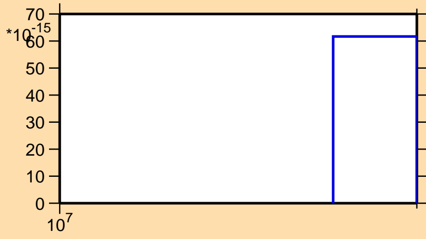
\sigma vs. E for ^{116}\text{Sn}(n,nt)
