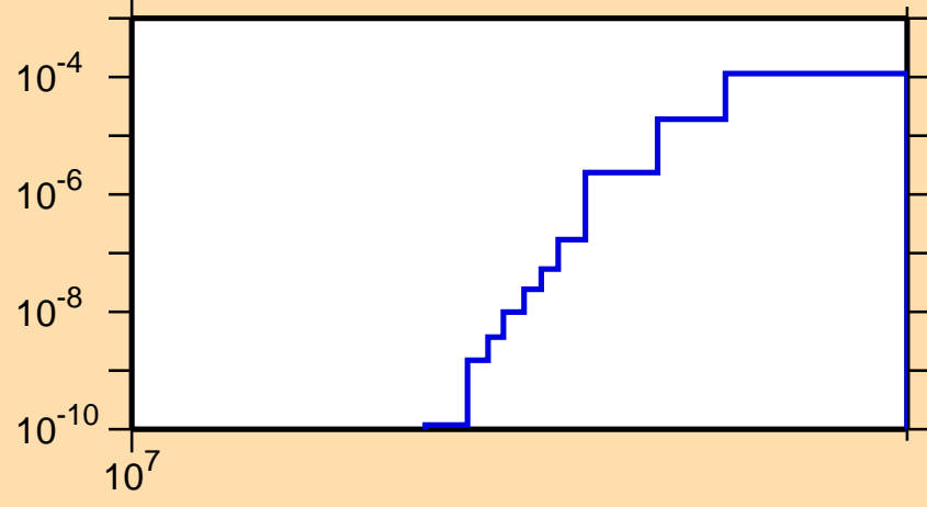
\sigma vs. E for ^{116}\text{Sn}(n,t)
