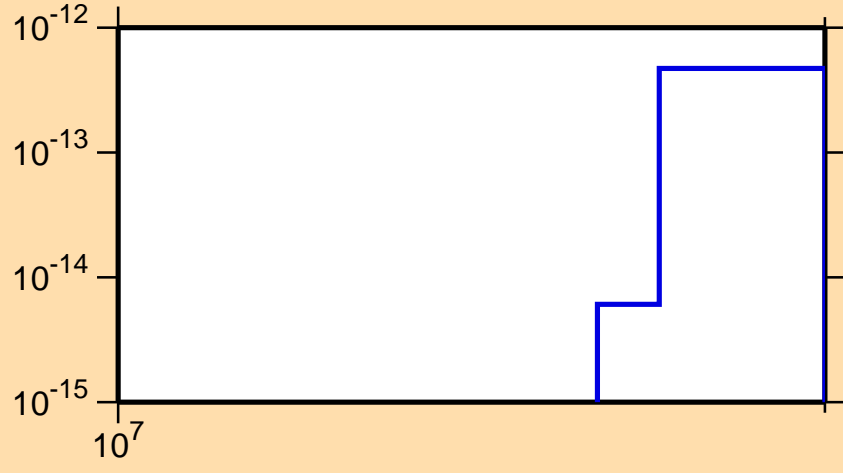
\sigma vs. E for ^{116}\text{Sn}(n,p\alpha)
