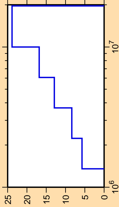
\Delta\sigma/\sigma vs. E for ^{116}\text{Sn}(n,n_2)
