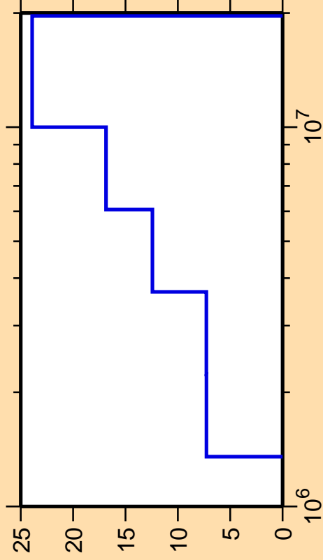
\Delta\sigma/\sigma vs. E for ^{116}\text{Sn}(n,n_3)
