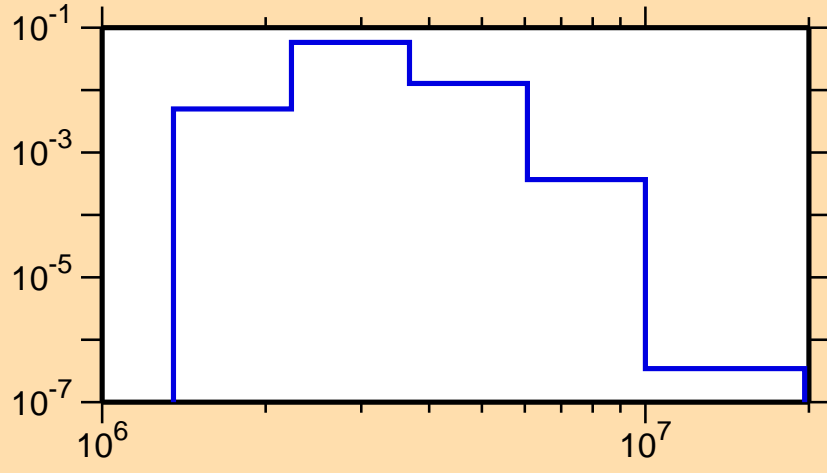
\sigma vs. E for ^{116}\text{Sn}(n,n_3)
