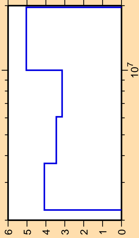
\Delta\sigma/\sigma vs. E for ^{116}\text{Sn}(n,n\text{cont.})
