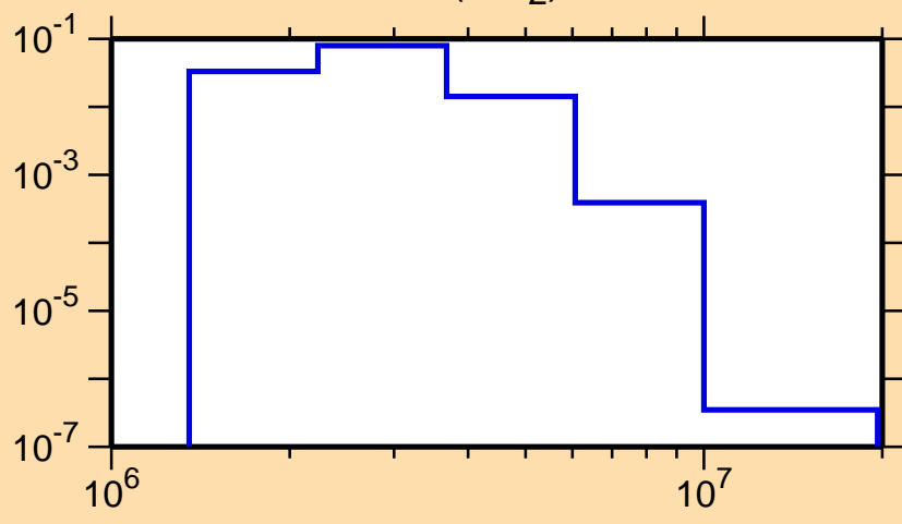
\sigma vs. E for ^{116}\text{Sn}(n,n_2)
