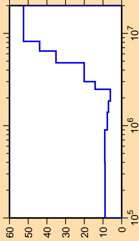
\Delta\sigma/\sigma vs. E for ^{117}\text{Sn}(n,n_3)
