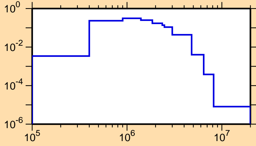
\sigma vs. E for ^{117}\text{Sn}(n,n_3)
