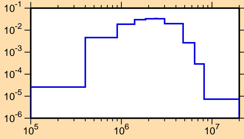
\sigma vs. E for ^{117}\text{Sn}(n,n_2)
