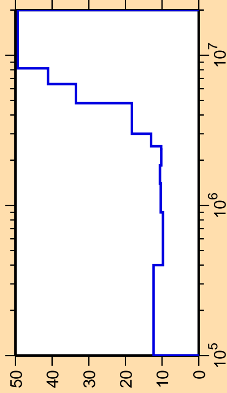
\Delta\sigma/\sigma vs. E for ^{117}\text{Sn}(n,n_2)
