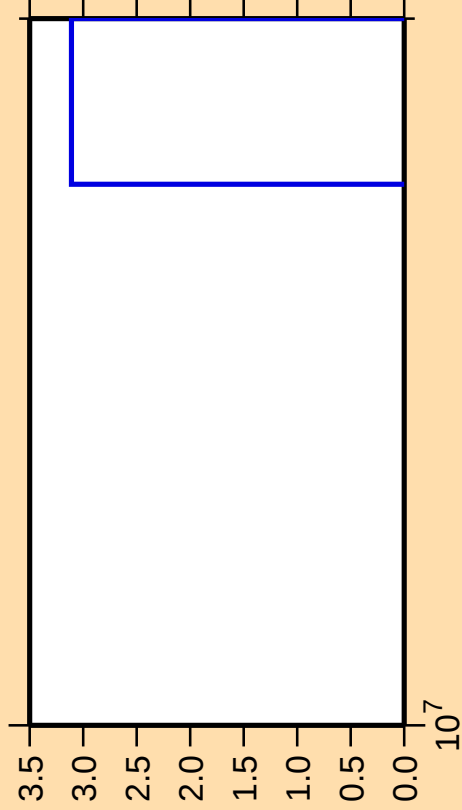
\Delta\sigma/\sigma vs. E for ^{120}\text{Sn}(n,\text{nd})
