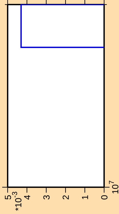
\Delta\sigma/\sigma vs. E for ^{120}\text{Sn}(n,2np)
