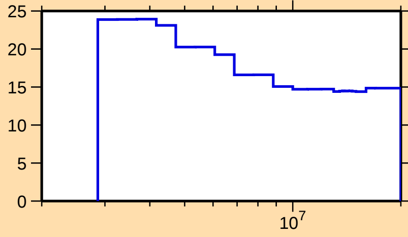
\Delta\sigma/\sigma vs. E for ^{120}\text{Sn}(n, n_1)
