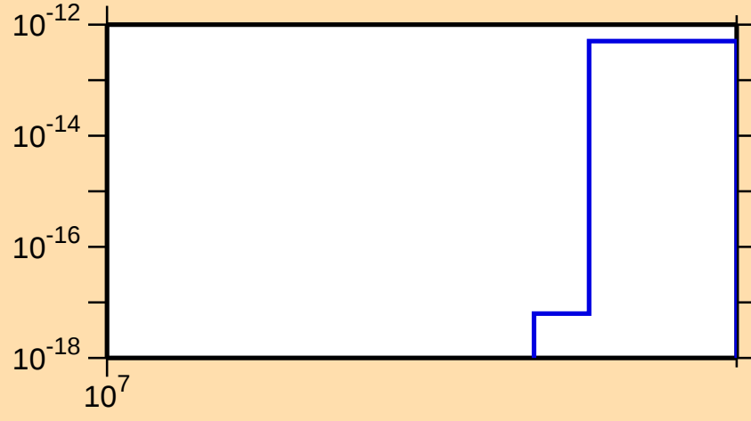
\sigma vs. E for ^{120}\text{Sn}(n,\text{He}3)
