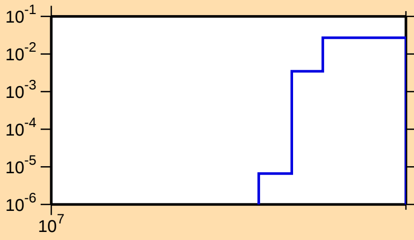
\sigma vs. E for ^{120}\text{Sn}(n,3n)
