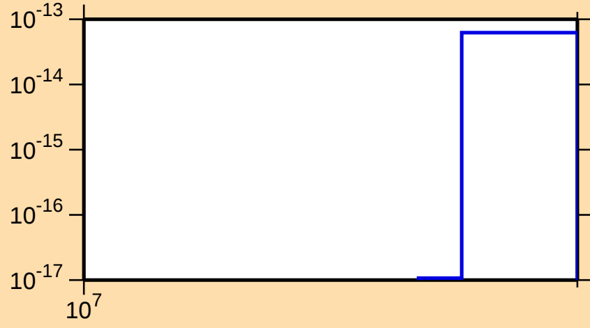
\sigma vs. E for ^{120}\text{Sn}(n,2n\alpha)
