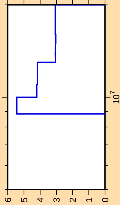
\Delta\sigma/\sigma vs. E for ^{120}\text{Sn}(n,2n)
