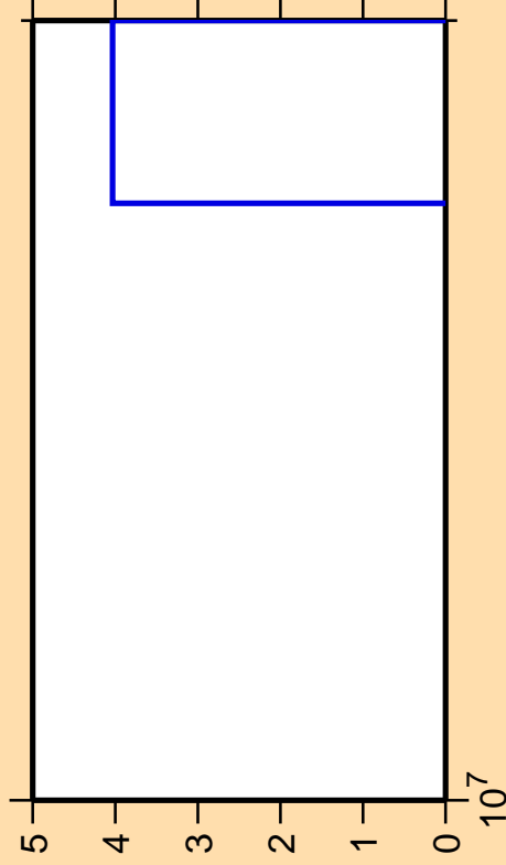
\Delta\sigma/\sigma vs. E for ^{123}\text{Sn}(n,2np)
