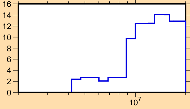
\Delta\sigma/\sigma vs. E for ^{123}\text{Sn}(n,n\text{cont.})
