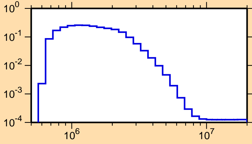
\sigma vs. E for ^{123}\text{Sn}(n,n_3)
