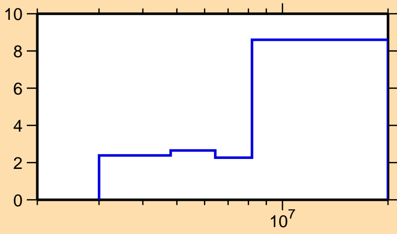
\Delta\sigma/\sigma vs. E for ^{123}\text{Sn}(n,n\text{cont.})
