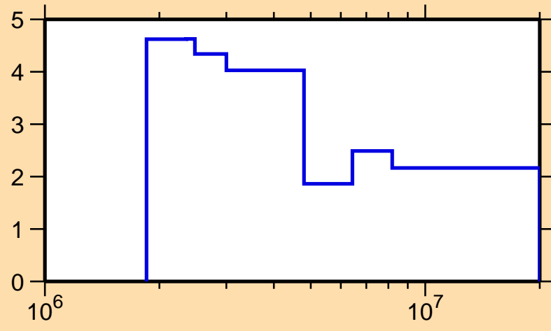
\Delta\sigma/\sigma vs. E for ^{123}\text{Sn}(n,\text{el.})
