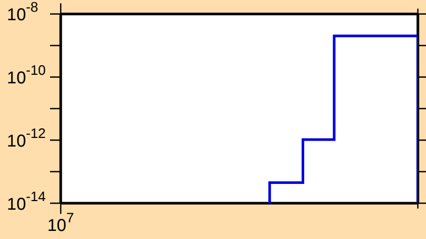
\sigma vs. E for ^{125}\text{Sn}(n,\text{nd})
