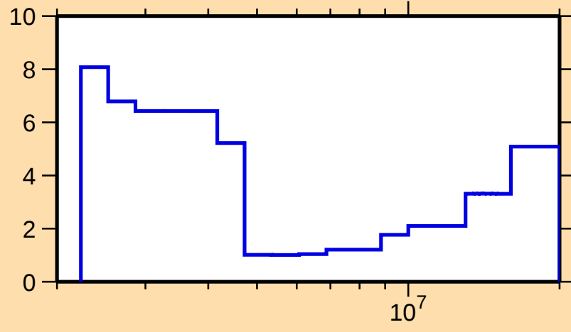
\Delta\sigma/\sigma vs. E for ^{125}\text{Sn}(n,\text{tot.})
