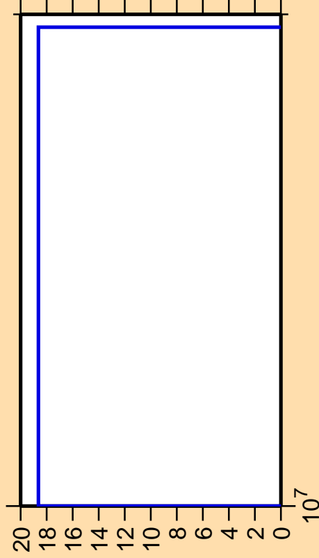
\Delta\sigma/\sigma vs. E for ^{125}\text{Sn}(n,nd)
