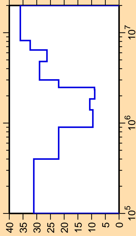
\Delta\sigma/\sigma vs. E for ^{125}\text{Sn}(n,n_2)
