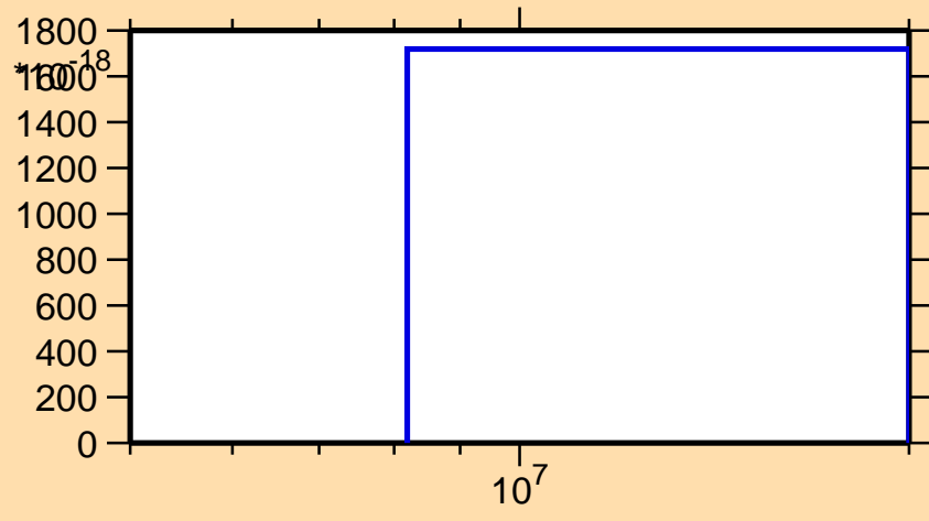
\sigma vs. E for ^{125}\text{Sn}(n,2n\alpha)
