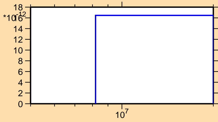
\sigma vs. E for ^{125}\text{Sn}(n,nd)
