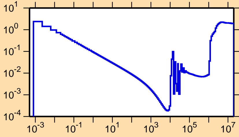
\sigma vs. E for ^{126}\text{Sn}(n,\text{nonel.})
