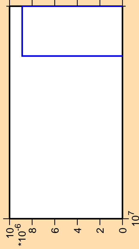
\Delta\sigma/\sigma vs. E for ^{126}\text{Sn}(n,nd)
