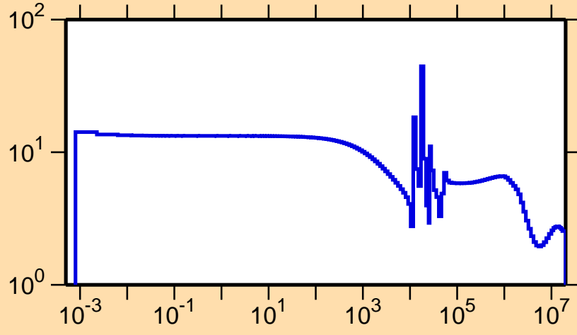
\sigma vs. E for ^{126}\text{Sn}(n,\text{el.})
