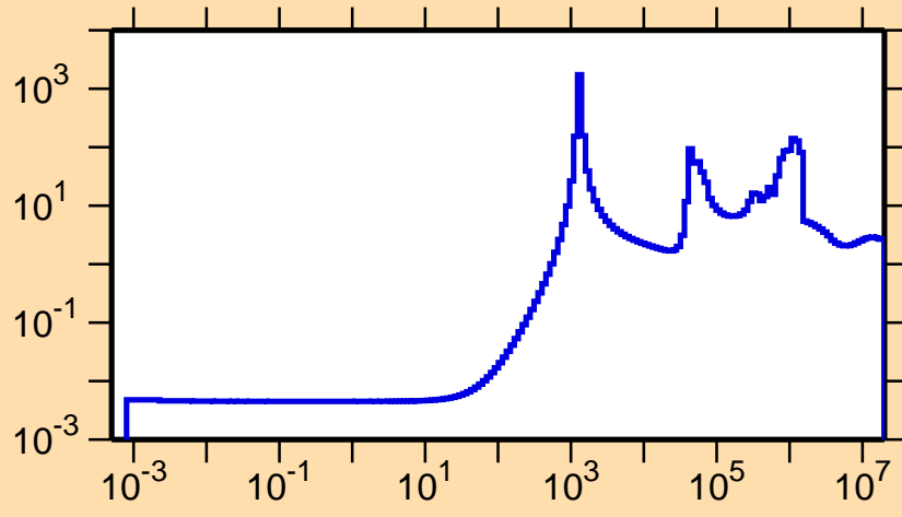
\sigma vs. E for ^{134}\text{Sn}(n,\text{el.})
