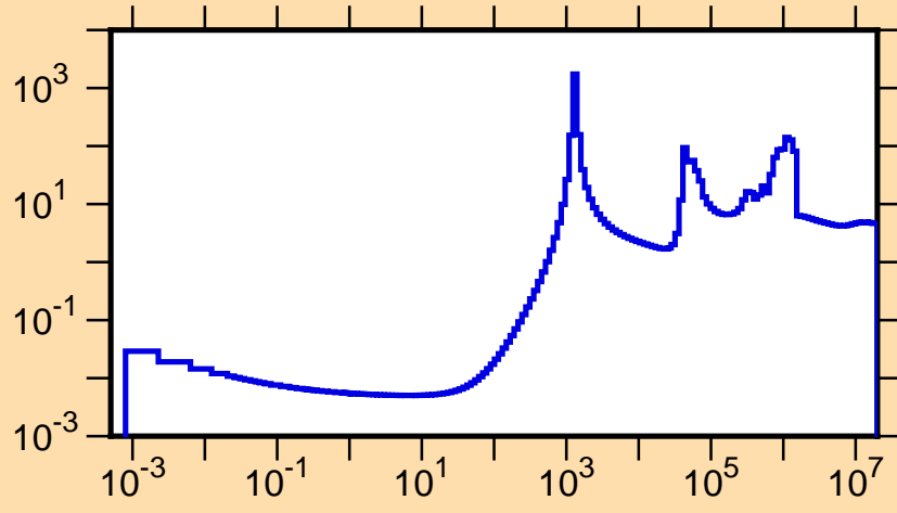
\sigma vs. E for ^{134}\text{Sn}(n,\text{tot.})
