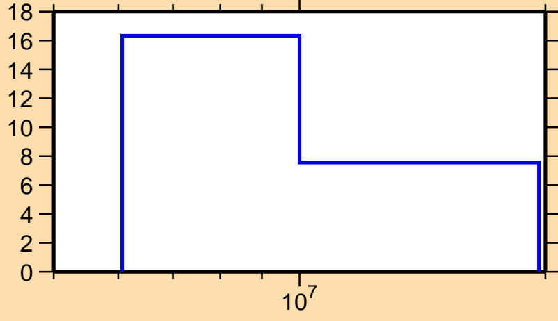
\Delta\sigma/\sigma vs. E for ^{134}\text{Sn}(n,\text{el.})
