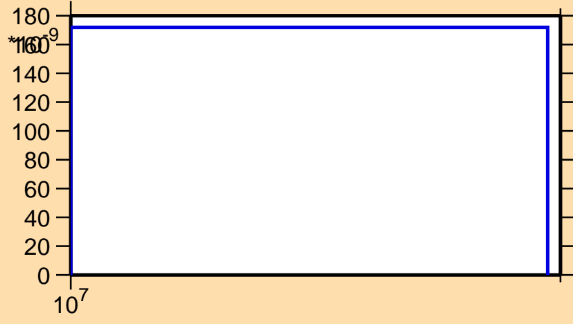
\sigma vs. E for ^{134}\text{Sn}(n,t)
