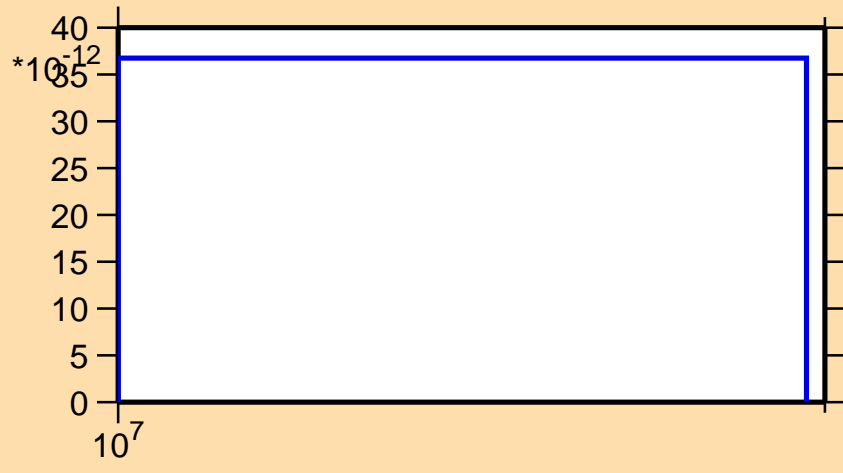
\sigma vs. E for ^{134}\text{Sn}(n,np)
