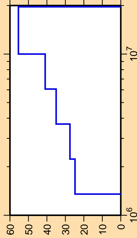
\Delta\sigma/\sigma vs. E for ^{134}\text{Sn}(n,\text{inel.})
