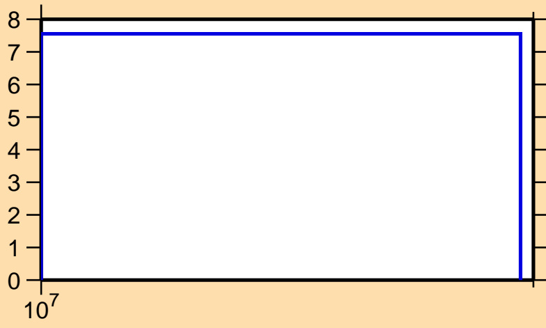
\Delta\sigma/\sigma vs. E for ^{134}\text{Sn}(n,\text{el.})
