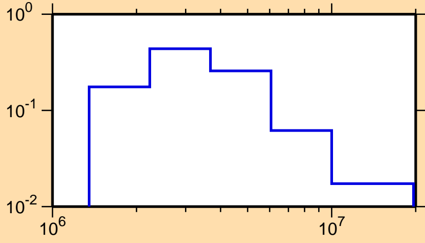
\sigma vs. E for ^{134}\text{Sn}(n,n_2)
