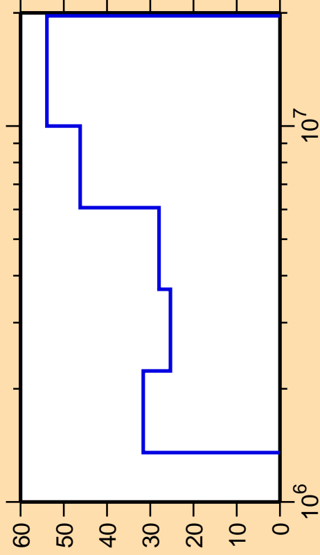
\Delta\sigma/\sigma vs. E for ^{134}\text{Sn}(n,n_2)
