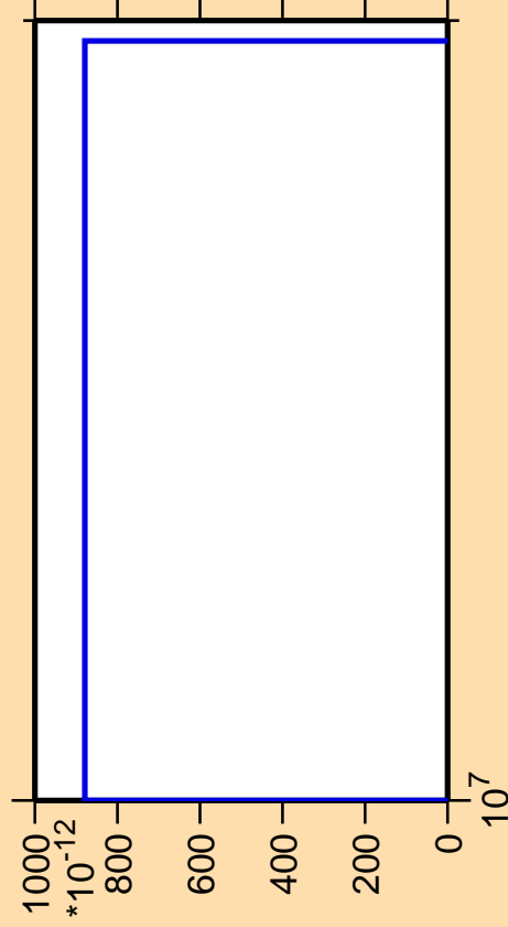
\Delta\sigma/\sigma vs. E for ^{134}\text{Sn}(n,2np)
