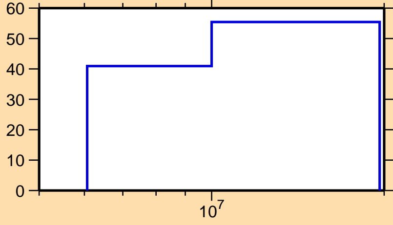
\Delta\sigma/\sigma vs. E for ^{134}\text{Sn}(n,\text{inel.})
