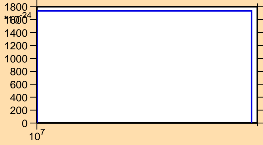
\sigma vs. E for ^{134}\text{Sn}(n,2np)
