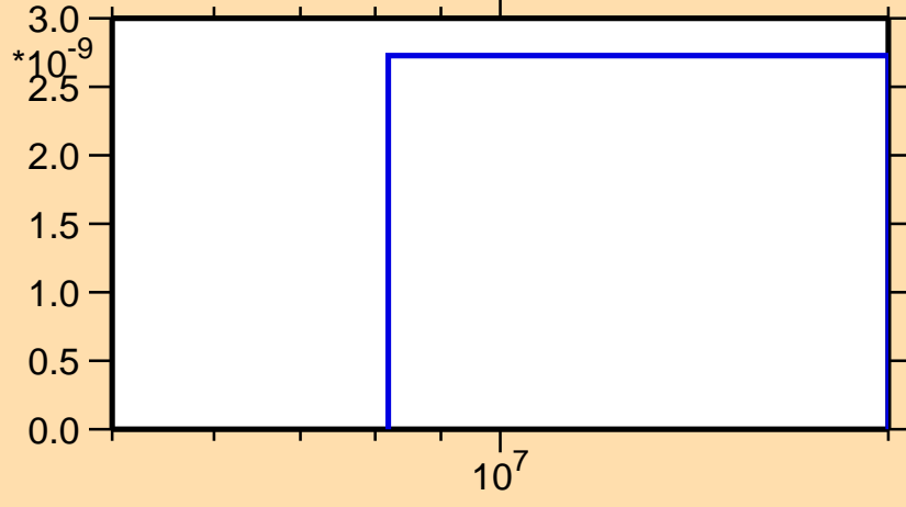
\sigma vs. E for ^{134}\text{Sn}(n,\alpha)
