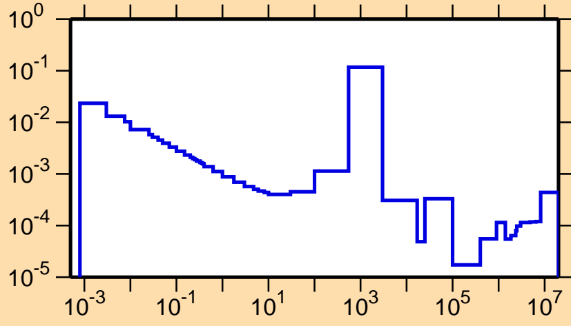
\sigma vs. E for ^{134}\text{Sn}(n,\gamma)
