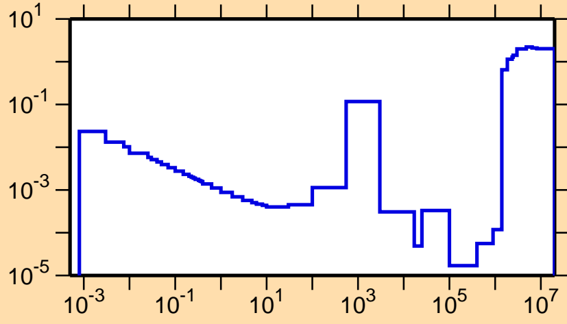
\sigma vs. E for ^{134}\text{Sn}(n,\text{nonel.})
