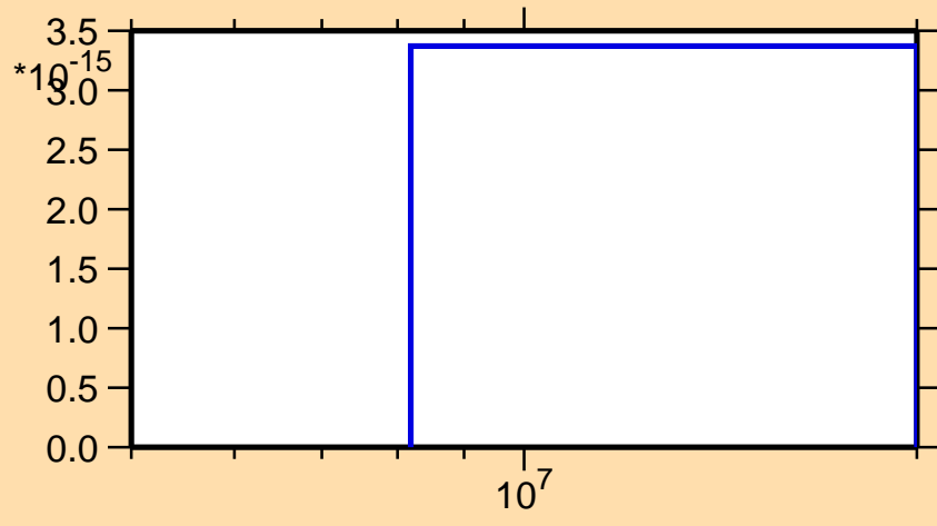
\sigma vs. E for ^{134}\text{Sn}(n,nd)
