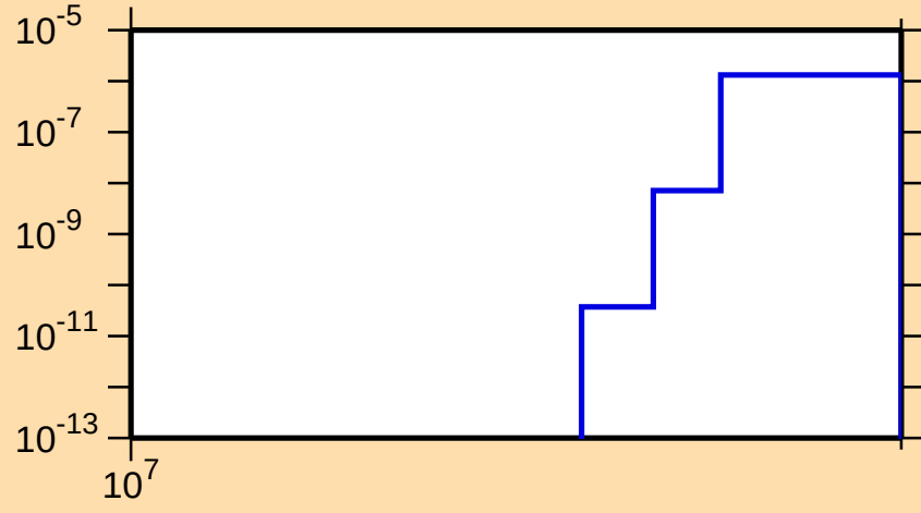
\sigma vs. E for ^{81}\text{Sr}(n,\text{pt})
