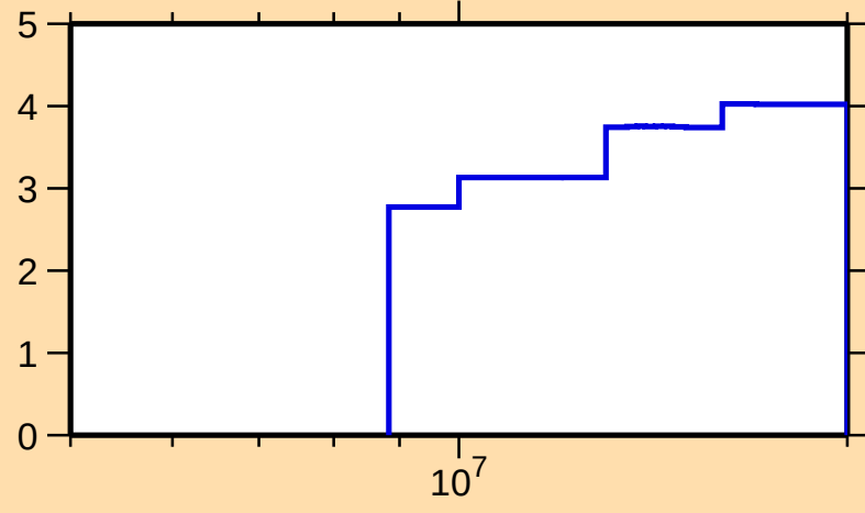
\Delta\sigma/\sigma vs. E for ^{81}\text{Sr}(n,\text{el.})
