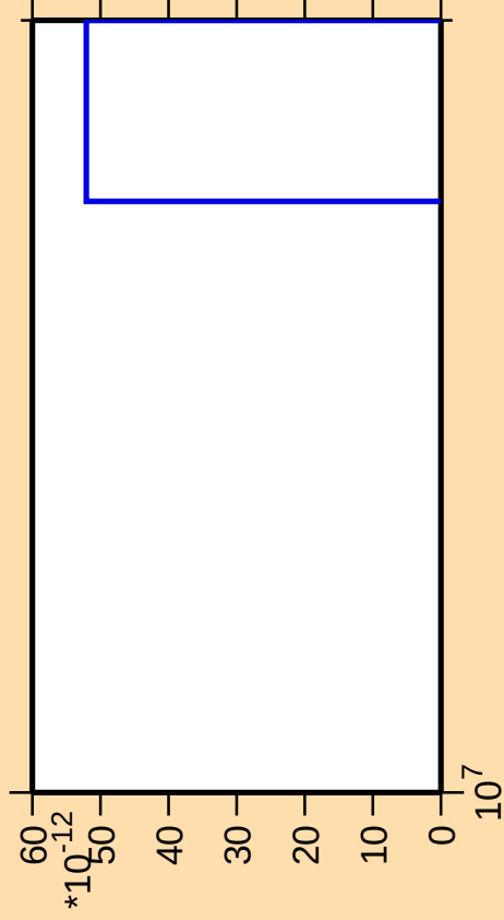
\Delta\sigma/\sigma vs. E for ^{81}\text{Sr}(n,\text{nt})
