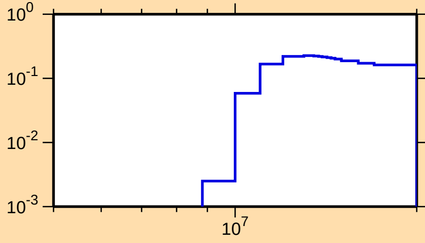
\sigma vs. E for ^{81}\text{Sr}(n,2n)
