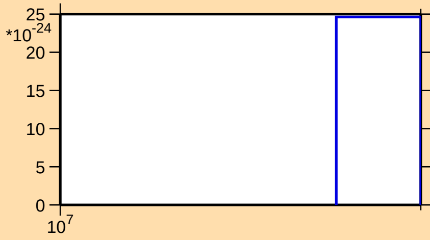
\sigma vs. E for ^{81}\text{Sr}(n,\text{nt})
