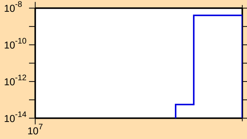
\sigma vs. E for ^{81}\text{Sr}(n,2n\alpha)
