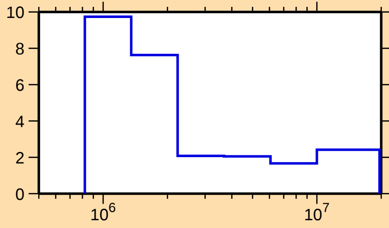
\Delta\sigma/\sigma vs. E for ^{81}\text{Sr}(n,\text{tot.})
