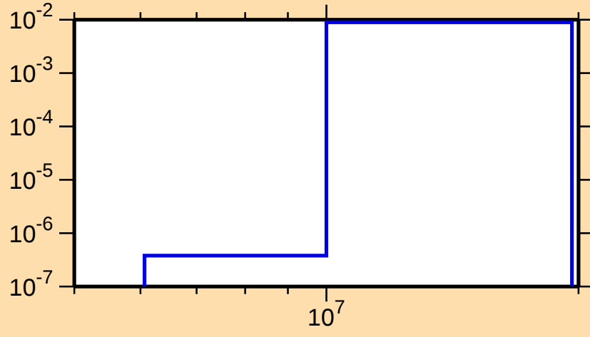
\sigma vs. E for ^{81}\text{Sr}(n,n\alpha)
