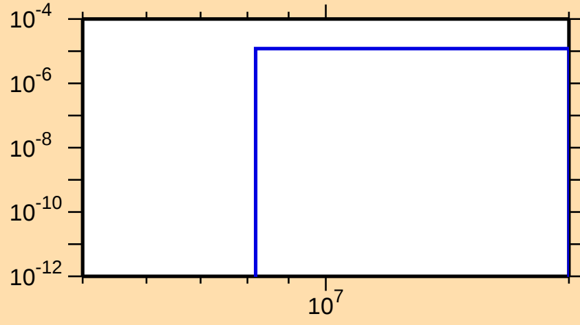
\sigma vs. E for ^{81}\text{Sr}(n,\text{He}3)
