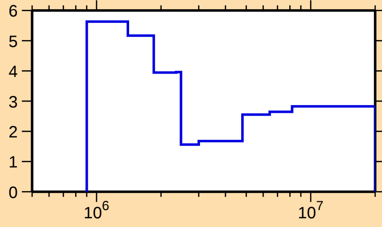
\Delta\sigma/\sigma vs. E for ^{81}\text{Sr}(n,\text{nonel.})
