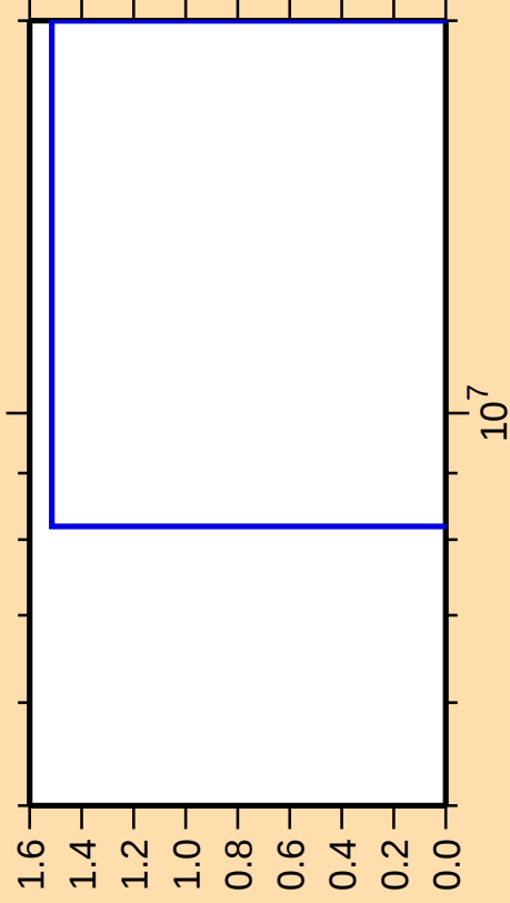
\Delta\sigma/\sigma vs. E for ^{81}\text{Sr}(\text{mt117})
