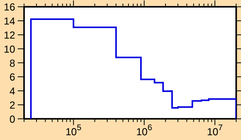
\Delta\sigma/\sigma vs. E for ^{81}\text{Sr}(n,\text{nonel.})
