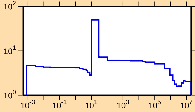
\sigma vs. E for ^{81}\text{Sr}(n,\text{el.})
