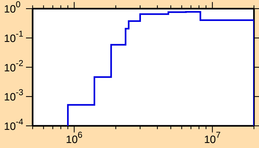
\sigma vs. E for ^{81}\text{Sr}(n,n\text{cont.})
