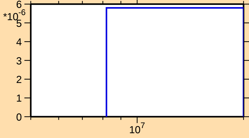
\sigma vs. E for ^{81}\text{Sr}(n,\text{pd})
