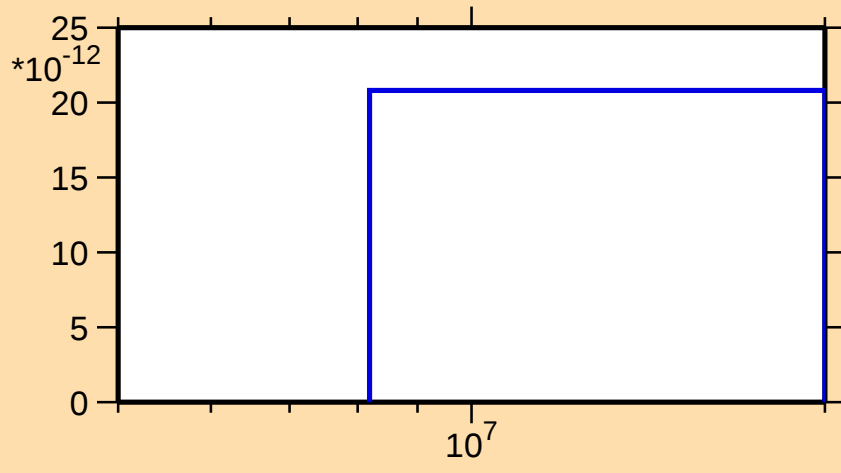
\sigma vs. E for ^{81}\text{Sr}(\text{mt } 34)
