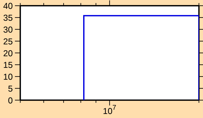
\Delta\sigma/\sigma vs. E for ^{81}\text{Sr}(n,2n)
