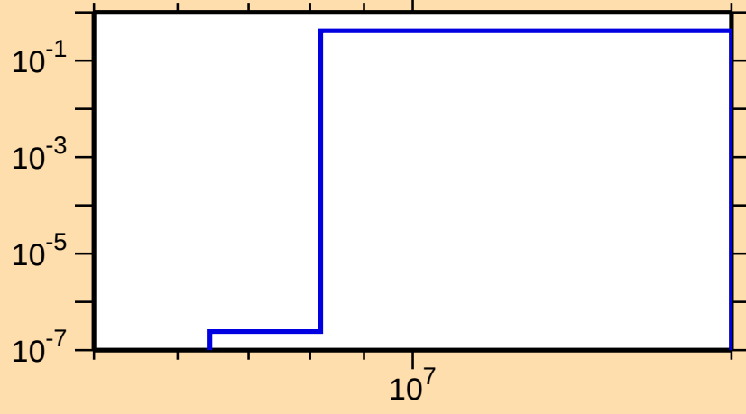
\sigma vs. E for ^{81}\text{Sr}(n,np)
