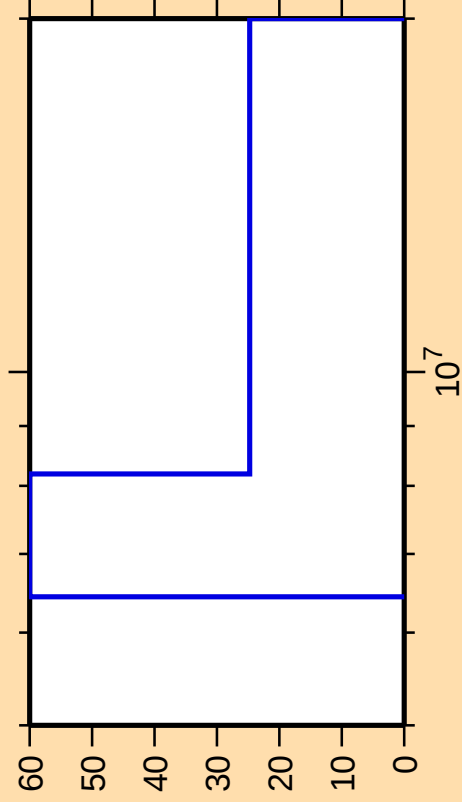
\Delta\sigma/\sigma vs. E for ^{81}\text{Sr}(n,n\alpha)
