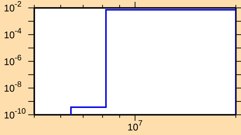
\sigma vs. E for ^{81}\text{Sr}(n,n\alpha)
