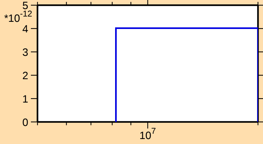
\sigma vs. E for ^{81}\text{Sr}(\text{mt } 45)
