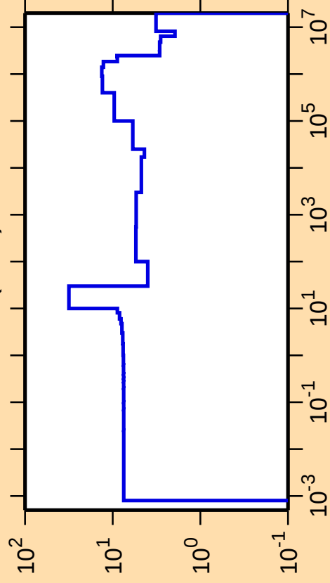
\Delta\sigma/\sigma vs. E for ^{81}\text{Sr}(n,\text{el.})
