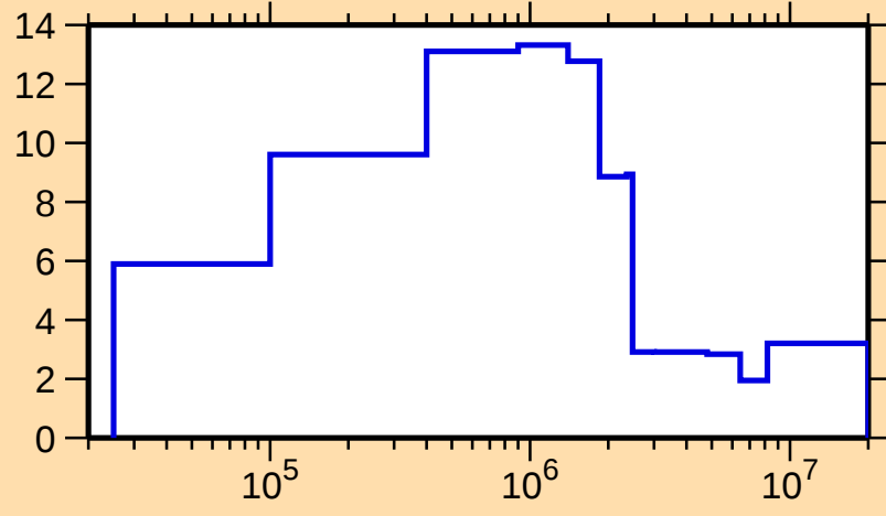
\Delta\sigma/\sigma vs. E for ^{81}\text{Sr}(n,\text{el.})
