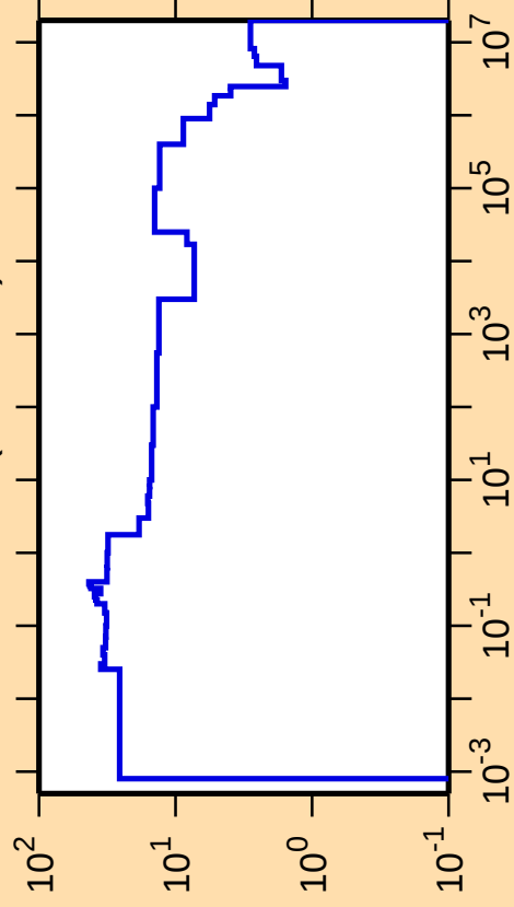
\Delta\sigma/\sigma vs. E for ^{81}\text{Sr}(n,\text{nonel.})
