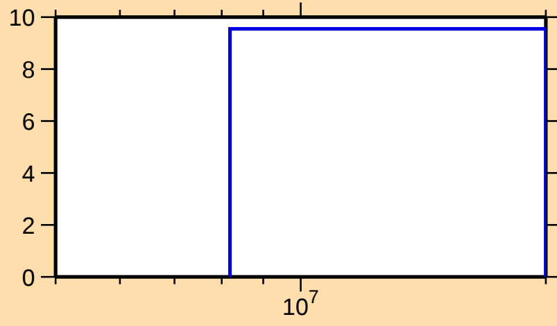
\Delta\sigma/\sigma vs. E for ^{81}\text{Sr}(n,\text{inel.})
