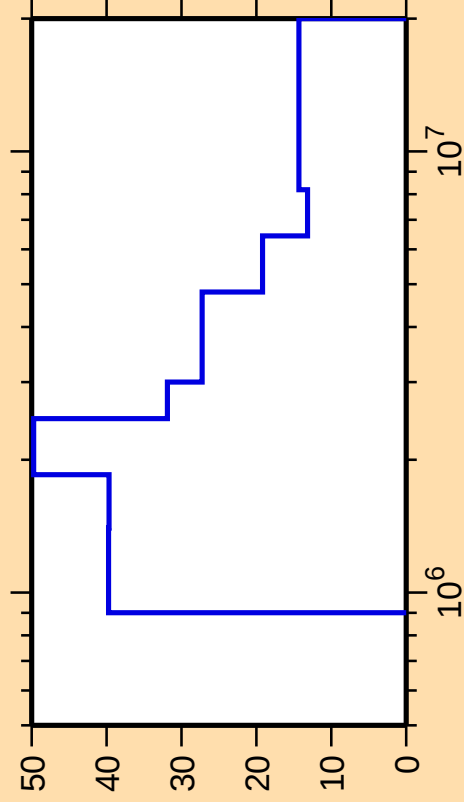
\Delta\sigma/\sigma vs. E for ^{81}\text{Sr}(n,\text{ncont.})
