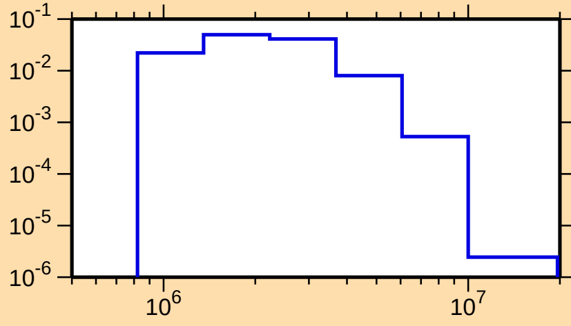
\sigma vs. E for ^{87}\text{Sr}(n,n_2)
