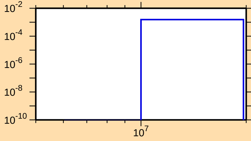
\sigma vs. E for ^{87}\text{Sr}(n,d)
