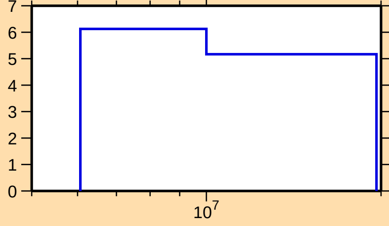
\Delta\sigma/\sigma vs. E for ^{87}\text{Sr}(n,2n)
