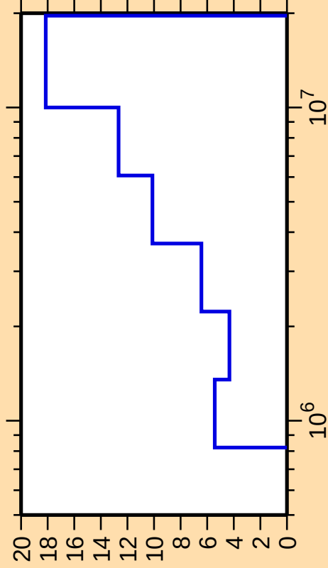
\Delta\sigma/\sigma vs. E for ^{87}\text{Sr}(n,n_2)
