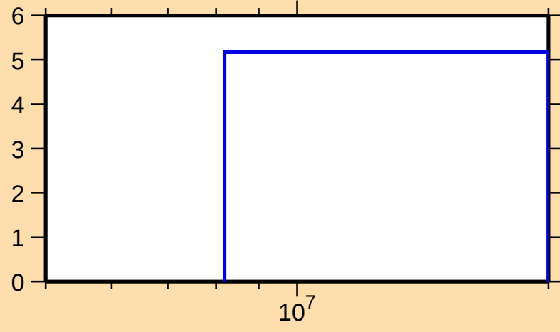
\Delta\sigma/\sigma vs. E for ^{87}\text{Sr}(n,2n)
