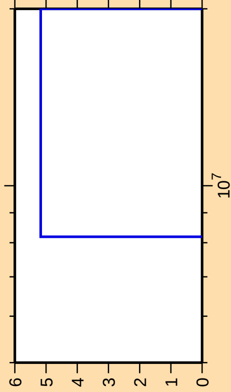
\Delta\sigma/\sigma vs. E for ^{87}\text{Sr}(n,2n)
