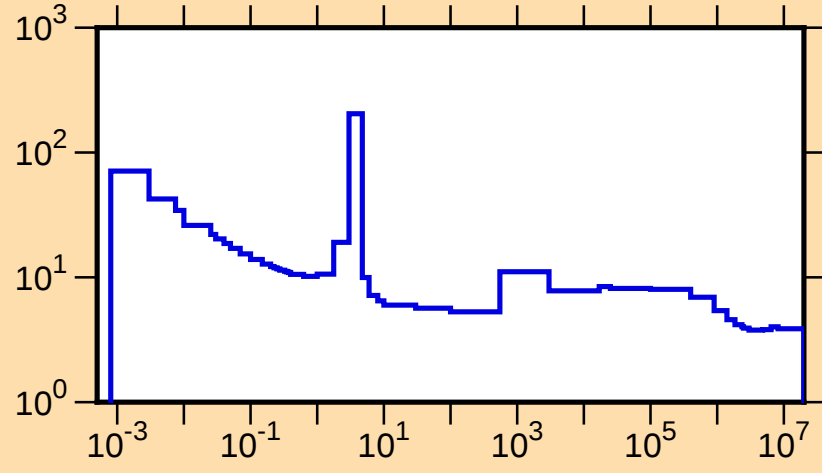
\sigma vs. E for ^{87}\text{Sr}(n,\text{tot.})
