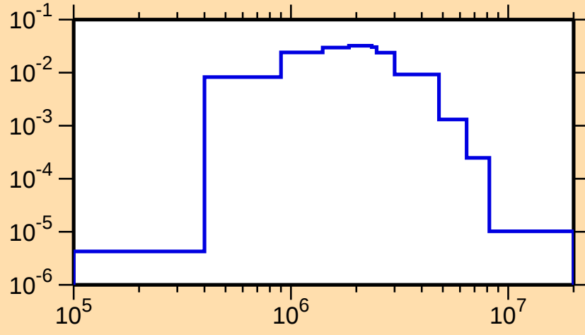
\sigma vs. E for ^{87}\text{Sr}(n,n_1)
