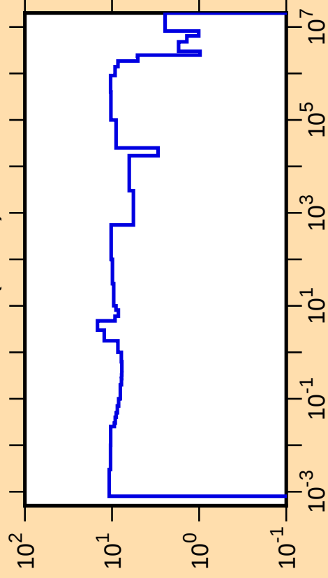
\Delta\sigma/\sigma vs. E for ^{87}\text{Sr}(n,\text{tot.})
