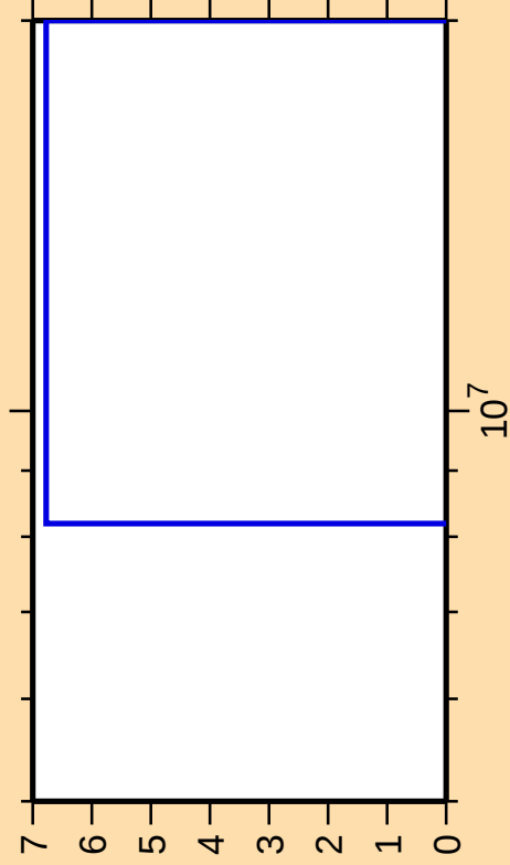
\Delta\sigma/\sigma vs. E for ^{87}\text{Sr}(n,n\text{cont.})
