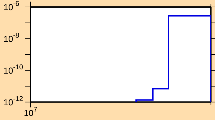
\sigma vs. E for ^{91}\text{Sr}(n,\text{nd})
