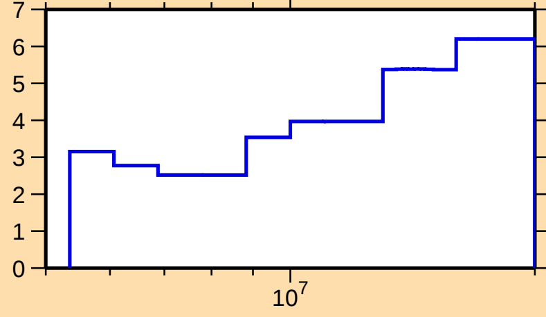
\Delta\sigma/\sigma vs. E for ^{91}\text{Sr}(n,\text{el.})
