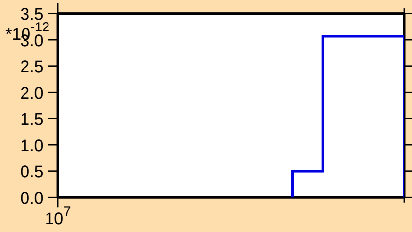
\sigma vs. E for ^{178}\text{Ta}(\text{mt117})
