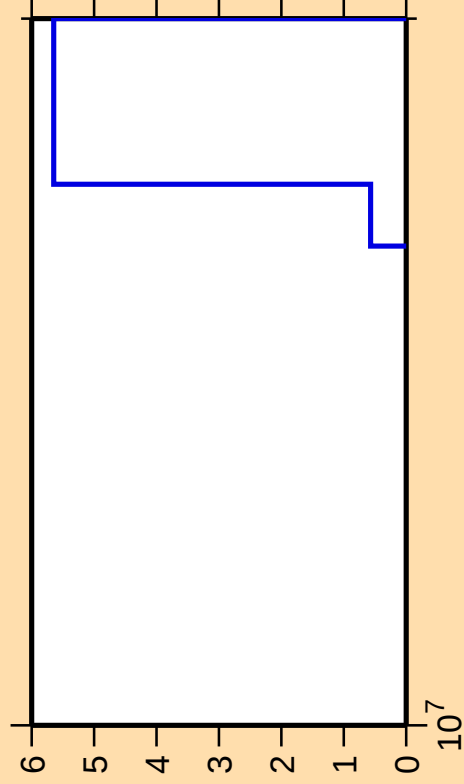
\Delta\sigma/\sigma vs. E for ^{178}\text{Ta}(\text{mt } 45)
