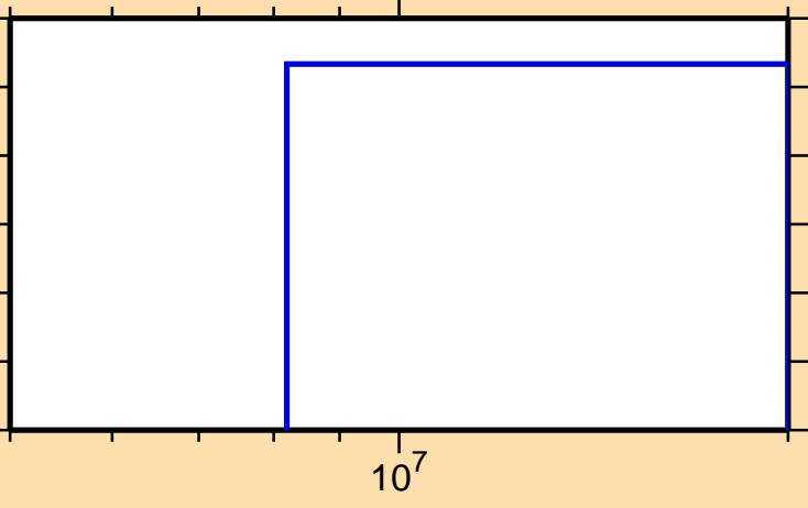
\sigma vs. E for ^{150}\text{Tb}(n,2np)
