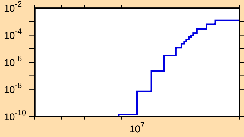
\sigma vs. E for ^{158}\text{Tb}(n,t)
