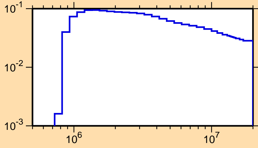
\sigma vs. E for ^{87}\text{Tc}(n,n_1)
