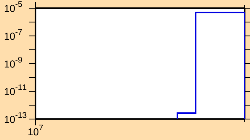
\sigma vs. E for ^{89}\text{Tc}(n,2np)
