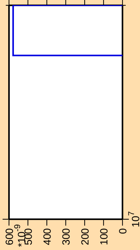
\Delta\sigma/\sigma vs. E for ^{89}\text{Tc}(n,\text{nt})
