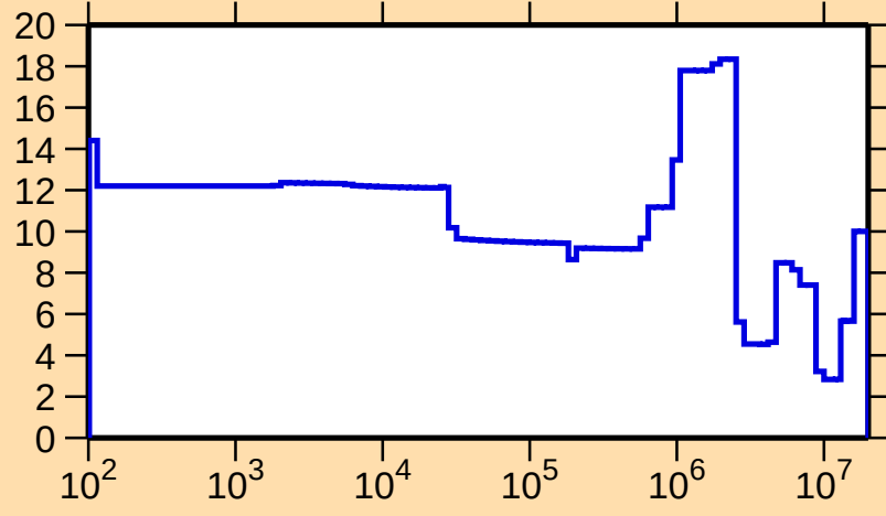
\Delta\sigma/\sigma vs. E for ^{89}\text{Tc}(n,\text{el.})
