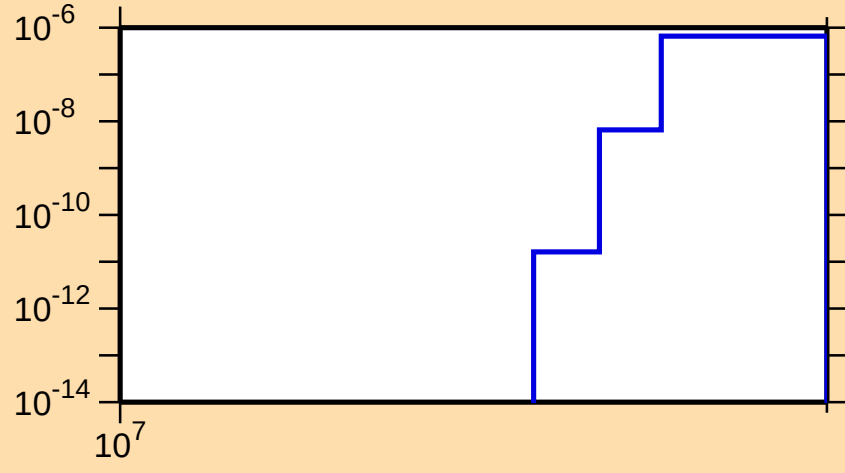
\sigma vs. E for ^{89}\text{Tc}(n,\text{nd})
