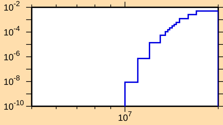
\sigma vs. E for ^{89}\text{Tc}(n,\text{pd})
