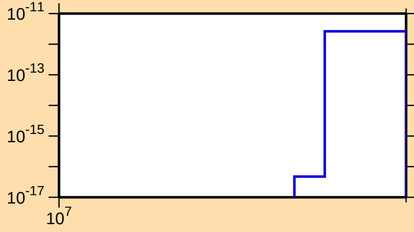
\sigma vs. E for ^{89}\text{Tc}(\text{mt } 34)
