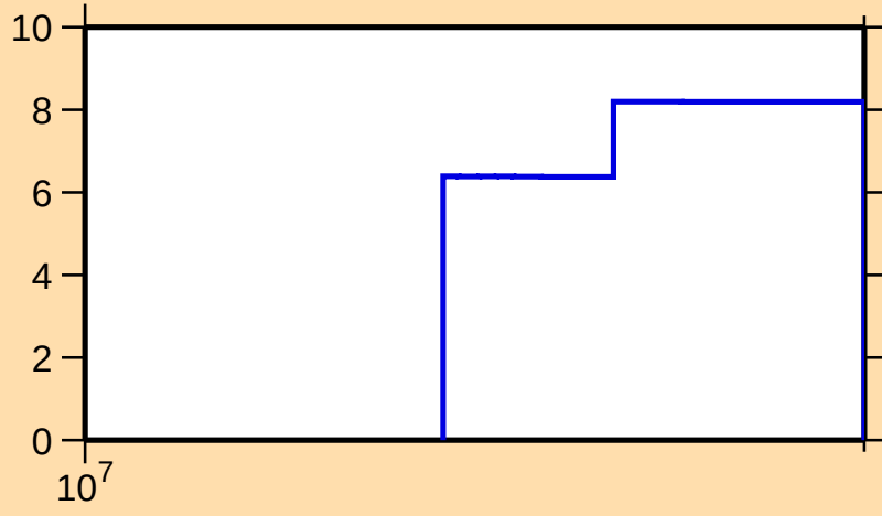
\Delta\sigma/\sigma vs. E for ^{89}\text{Tc}(n,\text{tot.})
