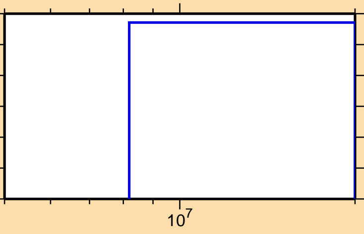
\sigma vs. E for ^{93}\text{Tc}(n,\text{nd})
