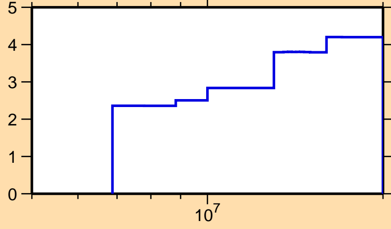
\Delta\sigma/\sigma vs. E for ^{98}\text{Tc}(n,\text{el.})
