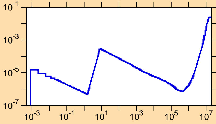
\sigma vs. E for ^{98}\text{Tc}(n,\alpha)
