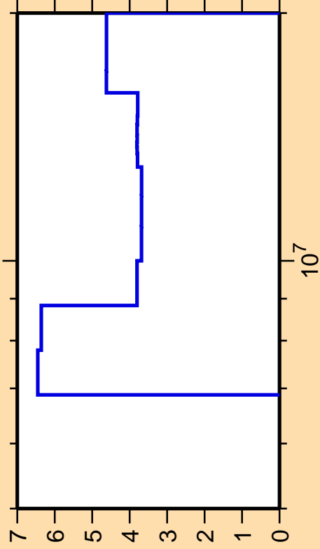
\Delta\sigma/\sigma vs. E for ^{98}\text{Tc}(n,2n)
