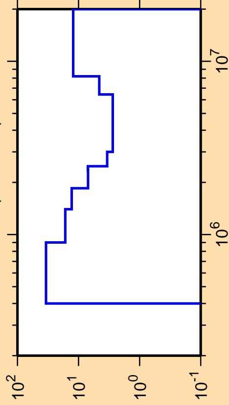
\Delta\sigma/\sigma vs. E for ^{98}\text{Tc}(n,n\text{cont.})
