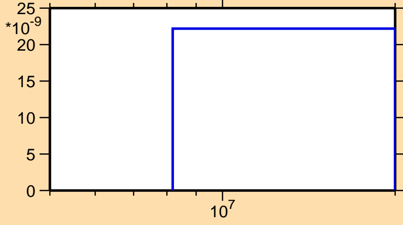
\sigma vs. E for ^{98}\text{Tc}(n,p\alpha)
