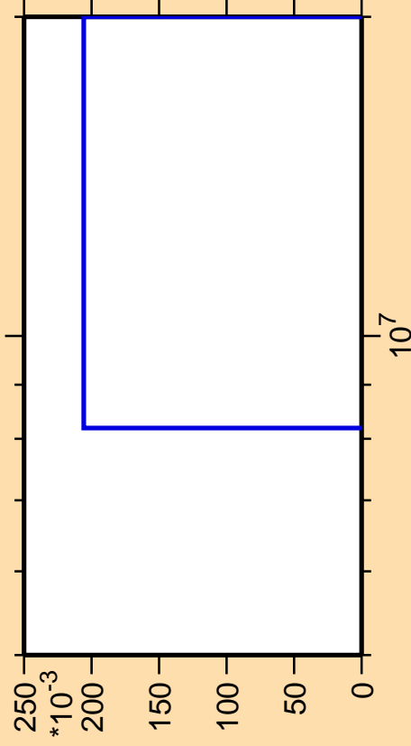
\Delta\sigma/\sigma vs. E for ^{98}\text{Tc}(\text{mt117})
