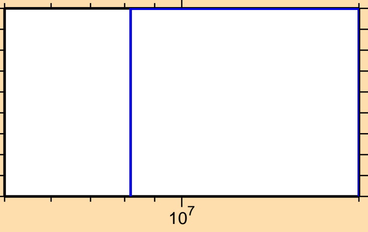
\sigma vs. E for ^{98}\text{Tc}(n,\text{He}3)
