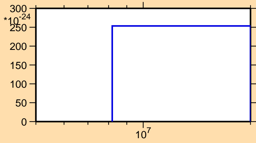
\sigma vs. E for ^{98}\text{Tc}(n,3n\alpha)
