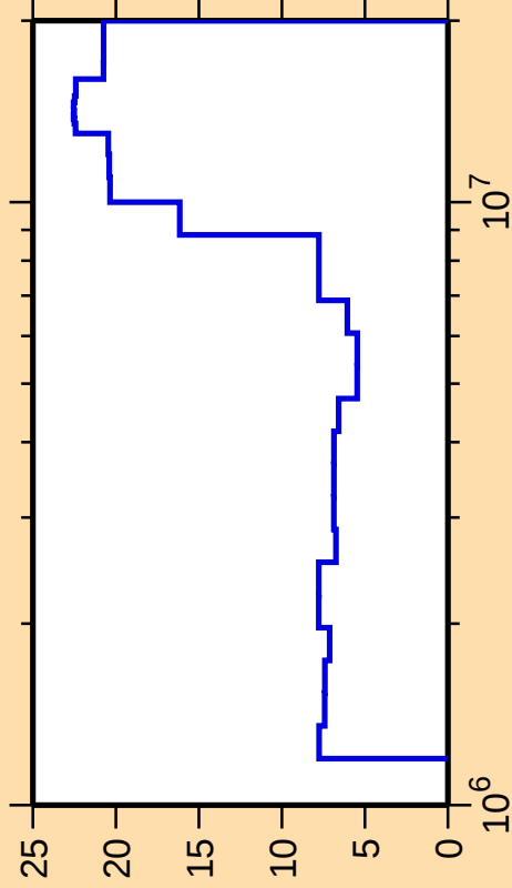
\Delta\sigma/\sigma vs. E for ^{103}\text{Tc}(n,n\text{cont.})
