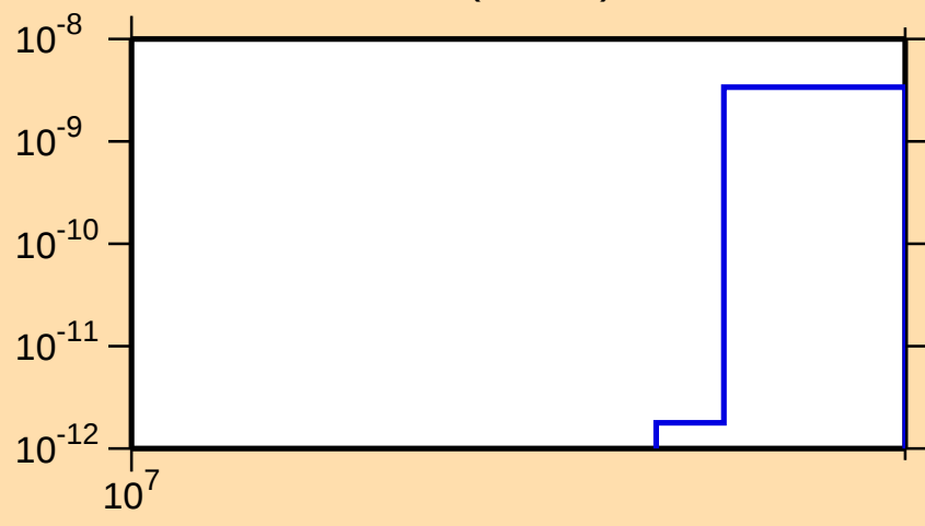
\sigma vs. E for ^{103}\text{Tc}(n,2n\alpha)
