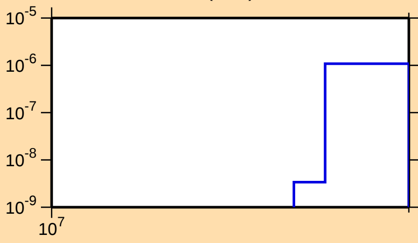
\sigma vs. E for ^{103}\text{Tc}(n,\text{nt})
