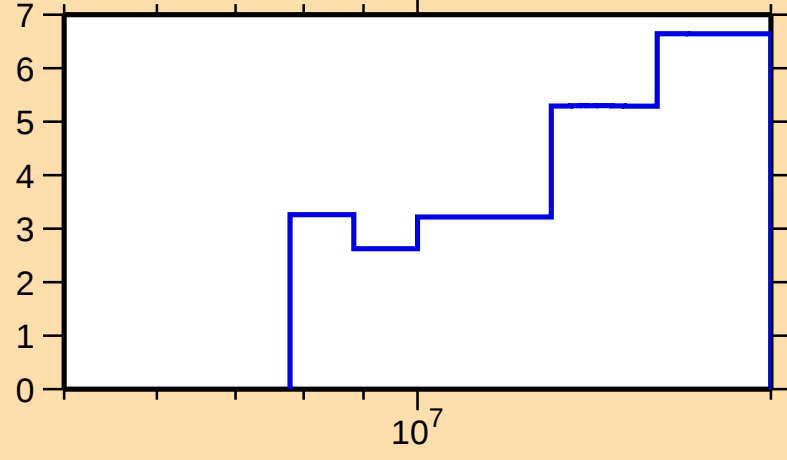
\Delta\sigma/\sigma vs. E for ^{103}\text{Tc}(n,\text{el.})
