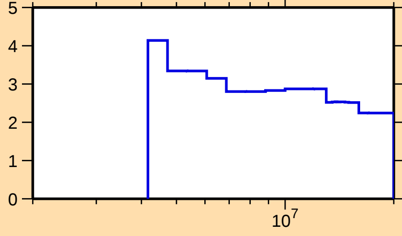
\Delta\sigma/\sigma vs. E for ^{103}\text{Tc}(n,\text{nonel.})
