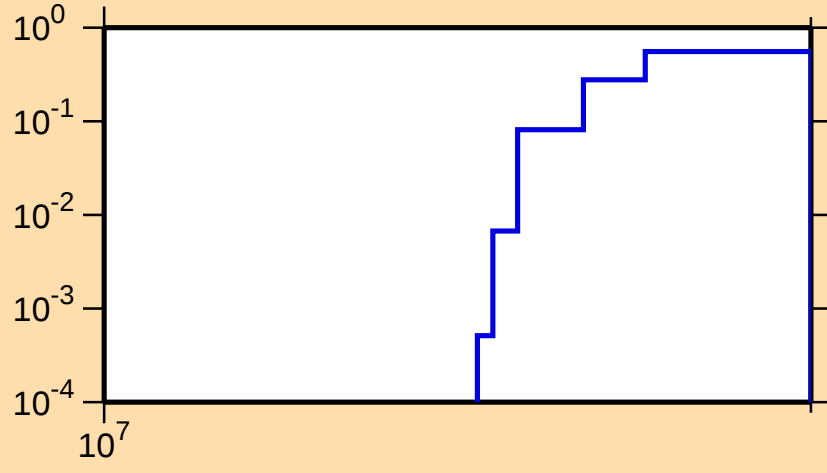
\sigma vs. E for ^{103}\text{Tc}(n,3n)
