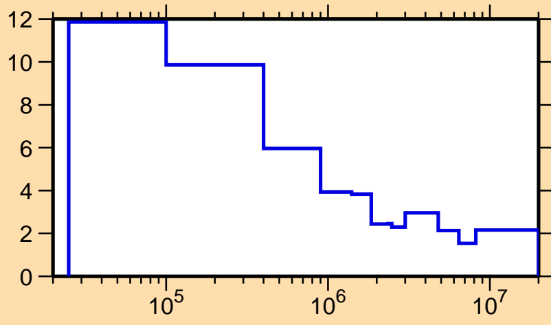
\Delta\sigma/\sigma vs. E for ^{103}\text{Tc}(n,\text{tot.})
