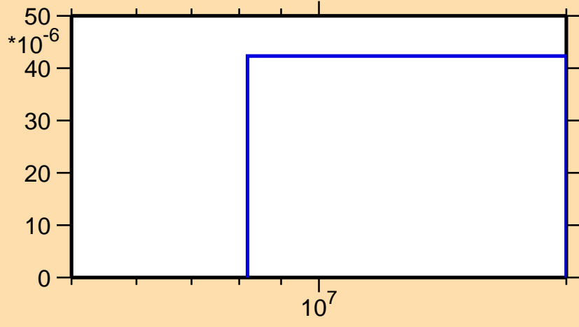
\sigma vs. E for ^{103}\text{Tc}(n,n\alpha)
