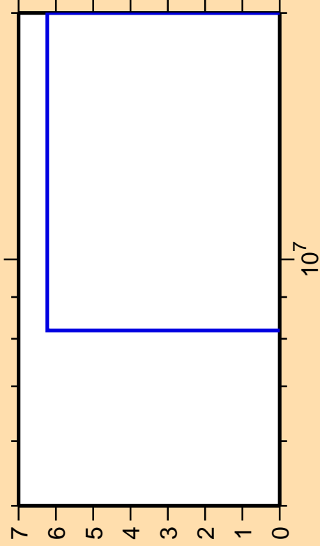
\Delta\sigma/\sigma vs. E for ^{103}\text{Tc}(n,3n)
