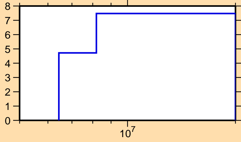
\Delta\sigma/\sigma vs. E for ^{103}\text{Tc}(n,\text{inel.})
