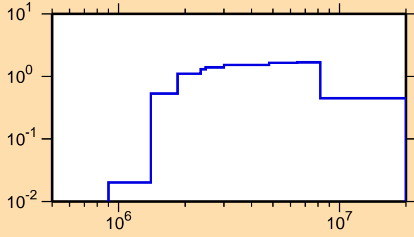
\sigma vs. E for ^{103}\text{Tc}(n,n\text{cont.})
