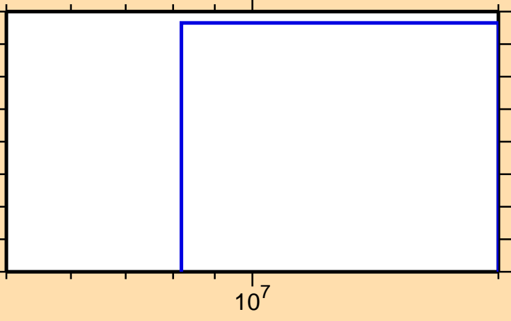
\sigma vs. E for ^{103}\text{Tc}(n,\text{nd})
