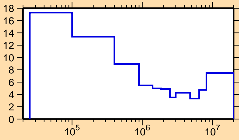
\Delta\sigma/\sigma vs. E for ^{103}\text{Tc}(n,\text{inel.})
