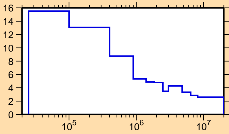
\Delta\sigma/\sigma vs. E for ^{103}\text{Tc}(n,\text{nonel.})
