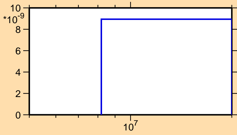
\sigma vs. E for ^{103}\text{Tc}(n,nt)
