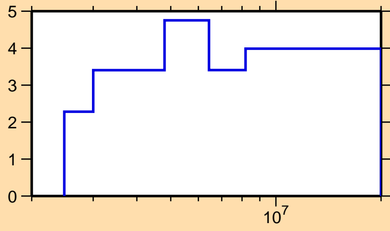
\Delta\sigma/\sigma vs. E for ^{103}\text{Tc}(n,el.)
