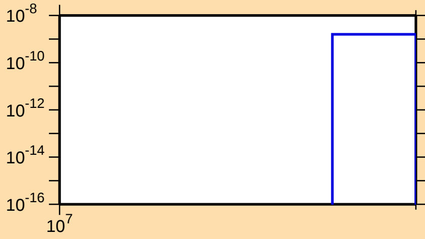
\sigma vs. E for ^{105}\text{Tc}(n,2np)
