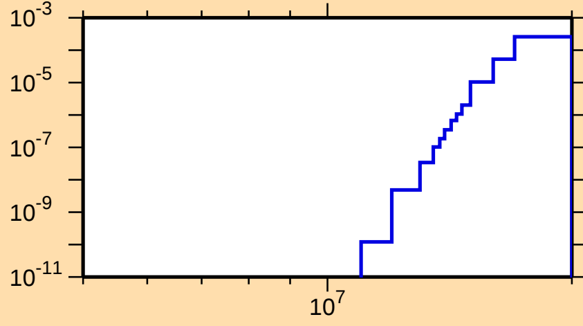
\sigma vs. E for ^{105}\text{Tc}(n,\alpha)
