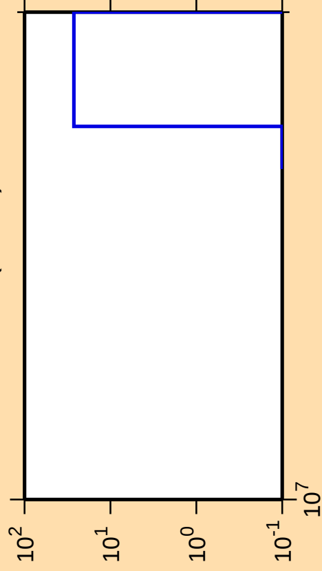
\Delta\sigma/\sigma vs. E for ^{105}\text{Tc}(n,2n\alpha)
