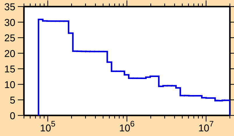
\Delta\sigma/\sigma vs. E for ^{105}\text{Tc}(n,\text{nonel.})
