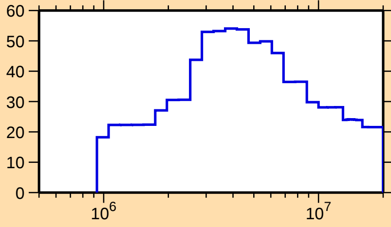
\Delta\sigma/\sigma vs. E for ^{105}\text{Tc}(n,n_1)
