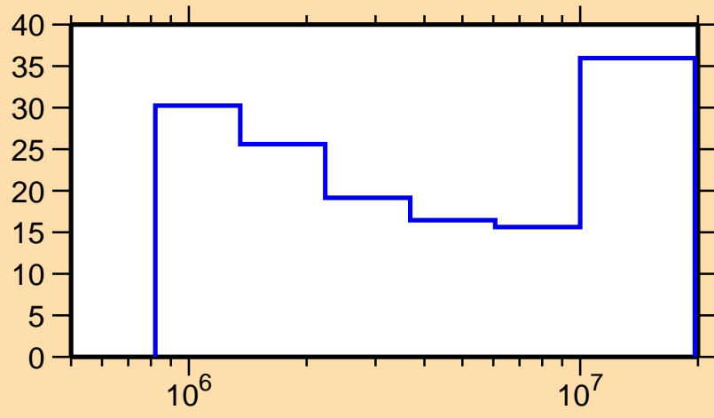
\Delta\sigma/\sigma vs. E for ^{105}\text{Tc}(n,n\text{cont.})
