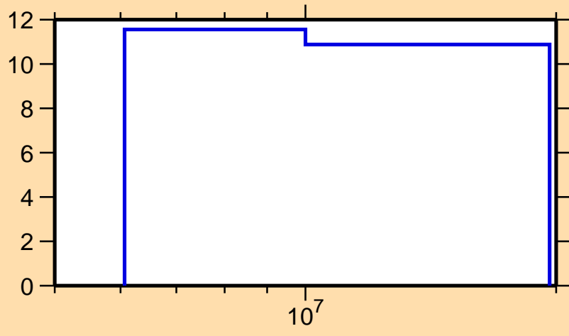
\Delta\sigma/\sigma vs. E for ^{105}\text{Tc}(n,2n)
