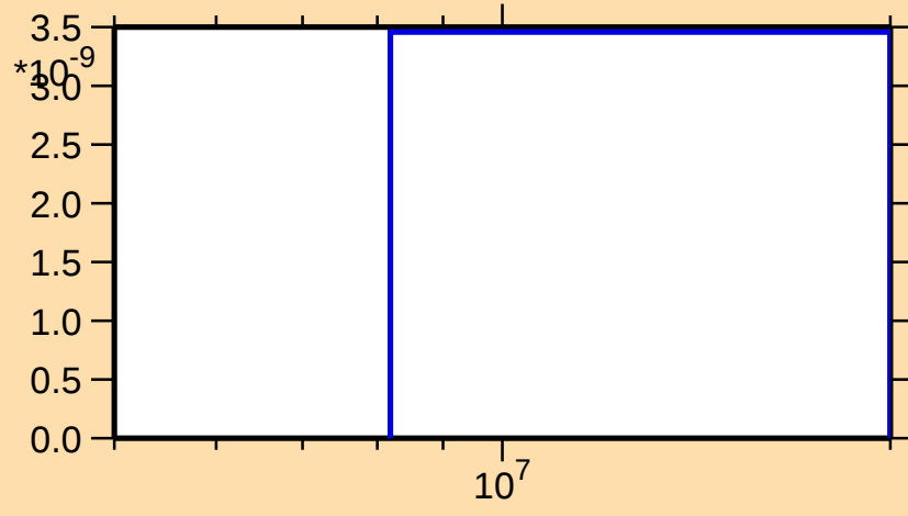
\sigma vs. E for ^{105}\text{Tc}(n,\text{nd})
