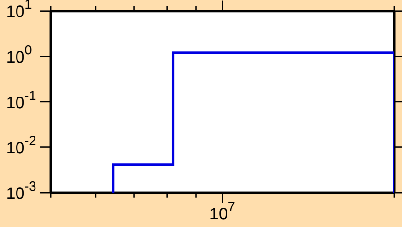
\sigma vs. E for ^{105}\text{Tc}(n,2n)
