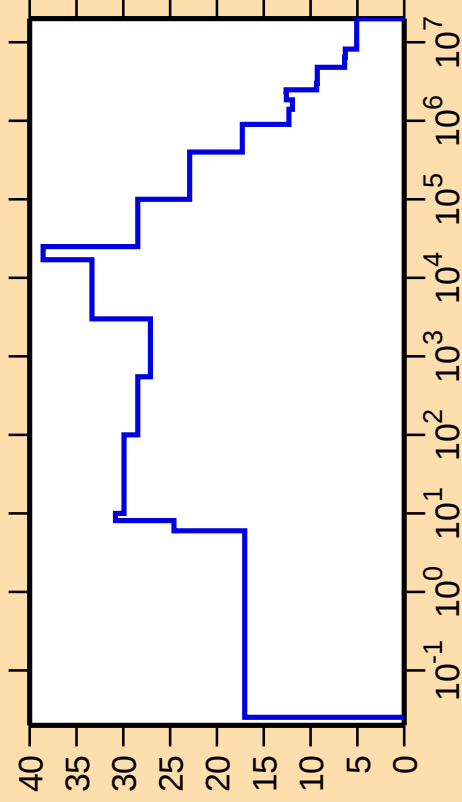
\Delta\sigma/\sigma vs. E for ^{105}\text{Tc}(n,\text{nonel.})
