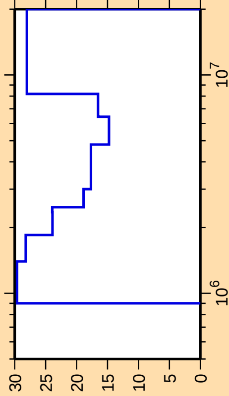
\Delta\sigma/\sigma vs. E for ^{105}\text{Tc}(n,\text{ncont.})
