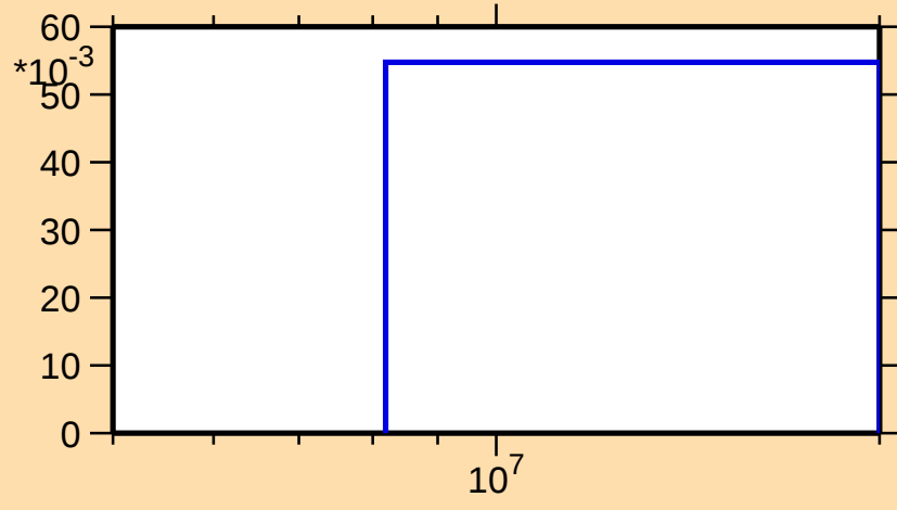
\sigma vs. E for ^{105}\text{Tc}(n,3n)
