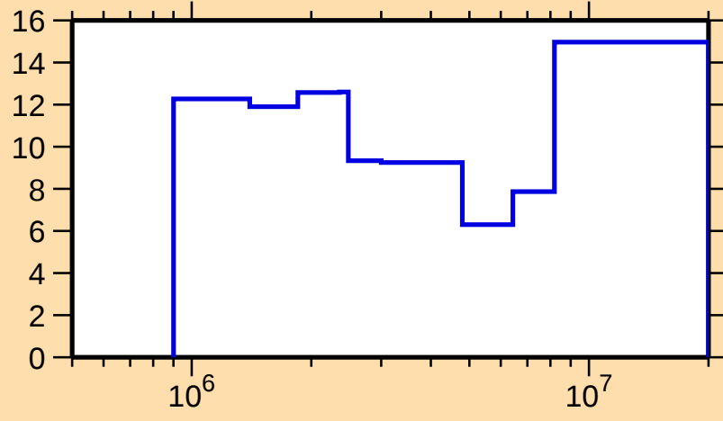
\Delta\sigma/\sigma vs. E for ^{105}\text{Tc}(n,\text{inel.})
