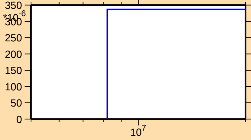
\sigma vs. E for ^{105}\text{Tc}(n,d)
