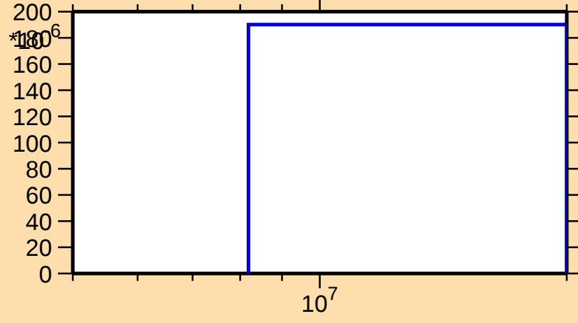
\sigma vs. E for ^{105}\text{Tc}(n,np)
