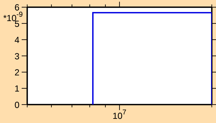
\sigma vs. E for ^{105}\text{Tc}(n,\text{nt})
