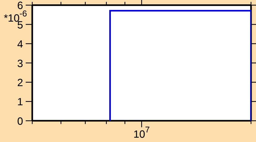
\sigma vs. E for ^{105}\text{Tc}(n,n\alpha)
