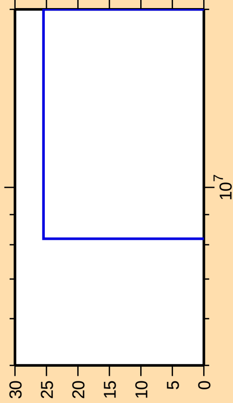
\Delta\sigma/\sigma vs. E for ^{105}\text{Tc}(n,np)
