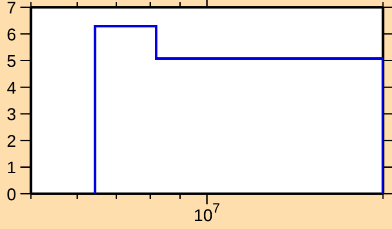
\Delta\sigma/\sigma vs. E for ^{105}\text{Tc}(n,\text{nonel.})
