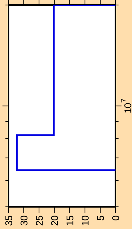
\Delta\sigma/\sigma vs. E for ^{105}\text{Tc}(n,p)
