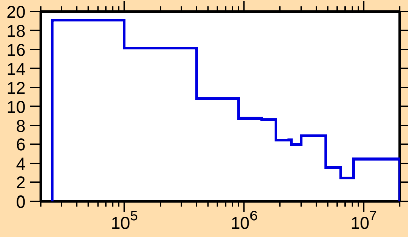
\Delta\sigma/\sigma vs. E for ^{105}\text{Tc}(n,\text{tot.})
