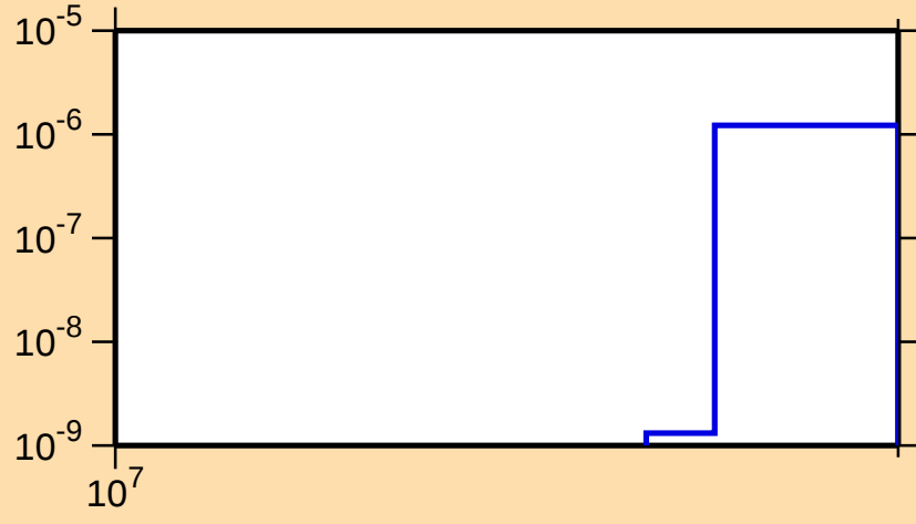
\sigma vs. E for ^{106}\text{Tc}(n,\text{nt})
