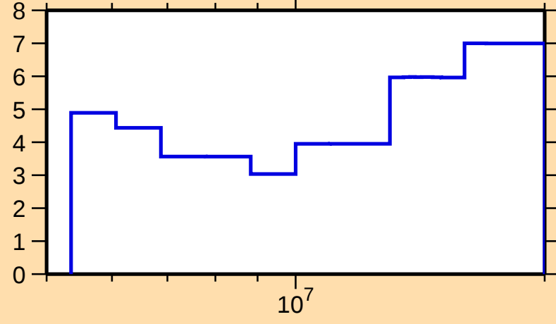
\Delta\sigma/\sigma vs. E for ^{106}\text{Tc}(n,\text{tot.})
