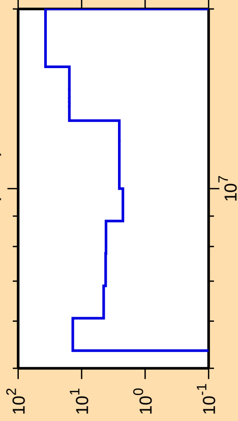
\Delta\sigma/\sigma vs. E for ^{106}\text{Tc}(n,2n)
