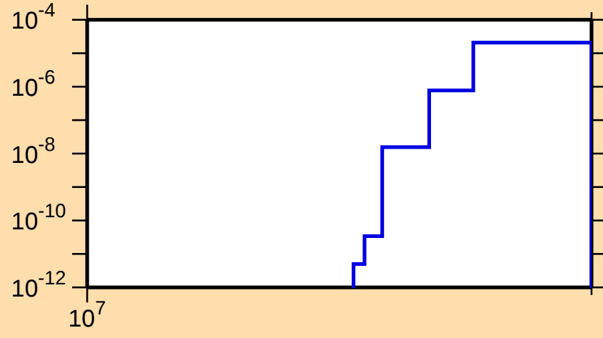
\sigma vs. E for ^{106}\text{Tc}(n,\text{nd})
