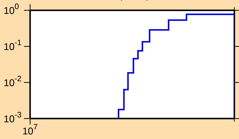
\sigma vs. E for ^{106}\text{Tc}(n,3n)
