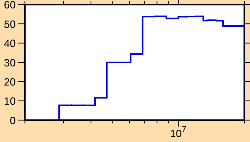
\Delta\sigma/\sigma vs. E for ^{106}\text{Tc}(n,n\text{cont.})
