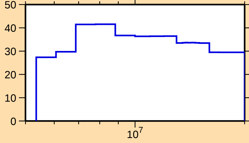
\Delta\sigma/\sigma vs. E for ^{106}\text{Tc}(n,\text{inel.})
