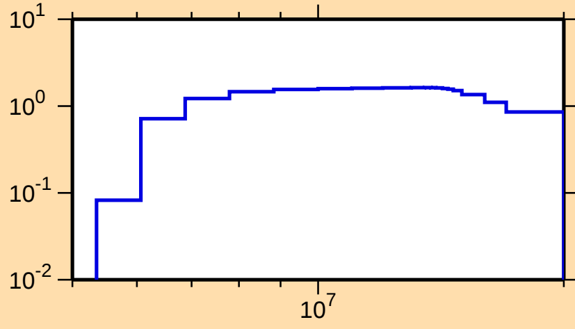
\sigma vs. E for ^{106}\text{Tc}(n,2n)
