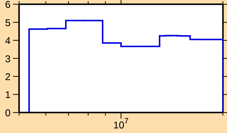
\Delta\sigma/\sigma vs. E for ^{106}\text{Tc}(n,\text{nonel.})
