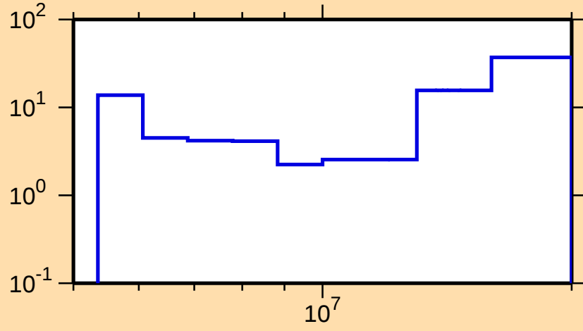
\Delta\sigma/\sigma vs. E for ^{106}\text{Tc}(n,2n)
