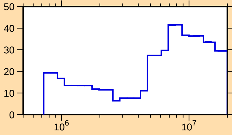
\Delta\sigma/\sigma vs. E for ^{106}\text{Tc}(n,\text{inel.})
