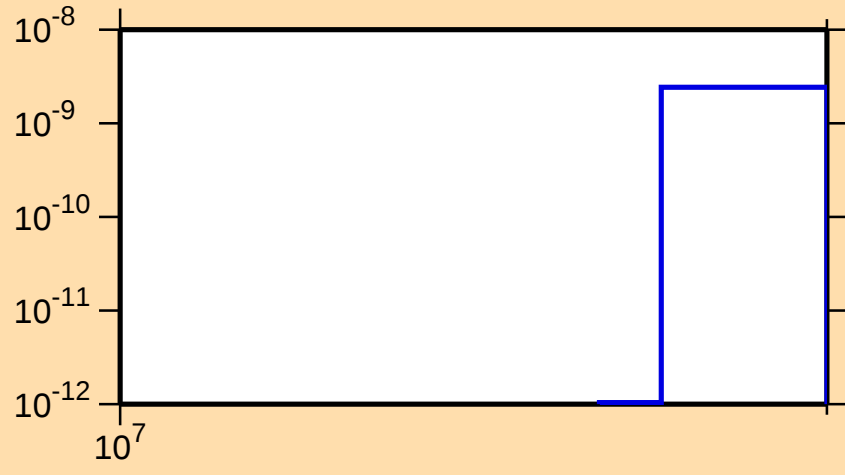
\sigma vs. E for ^{106}\text{Tc}(n,2n\alpha)
