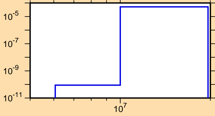
\sigma vs. E for ^{106}\text{Tc}(n,t)
