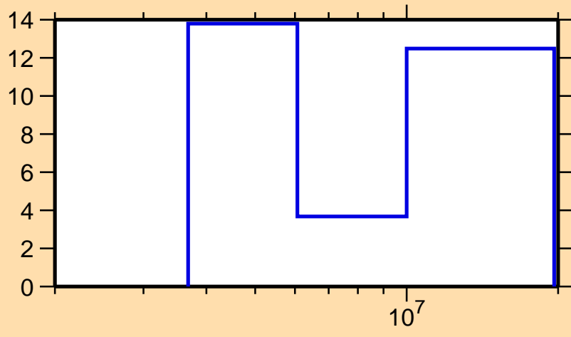
\Delta\sigma/\sigma vs. E for ^{106}\text{Tc}(n,2n)
