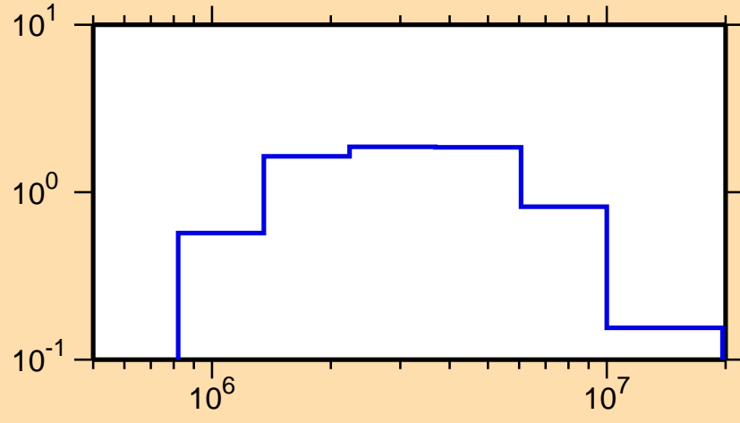
\sigma vs. E for ^{106}\text{Tc}(n,n\text{cont.})
