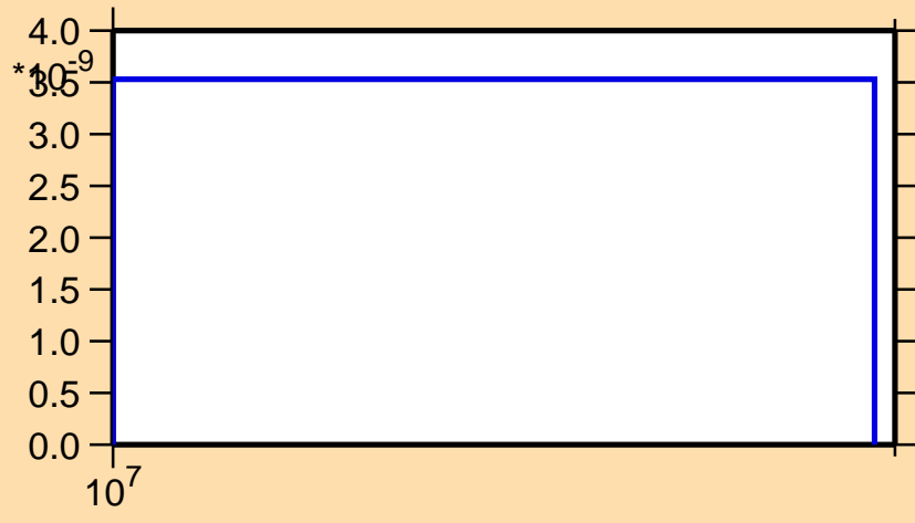
\sigma vs. E for ^{106}\text{Tc}(n,2np)
