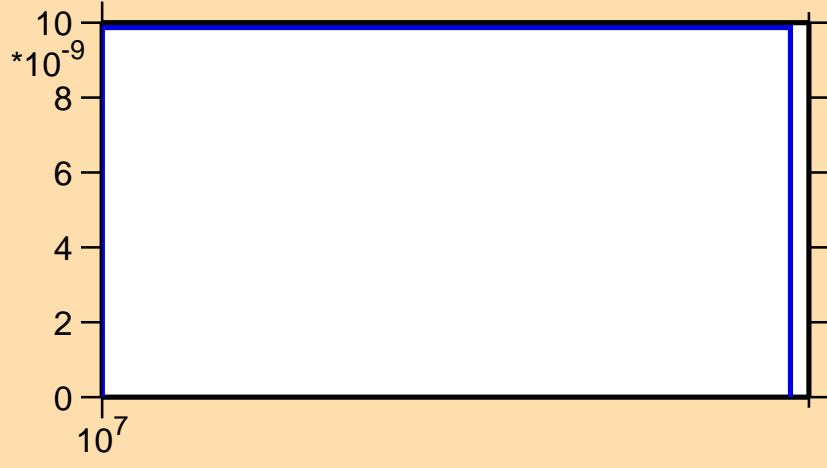
\sigma vs. E for ^{106}\text{Tc}(n,nt)
