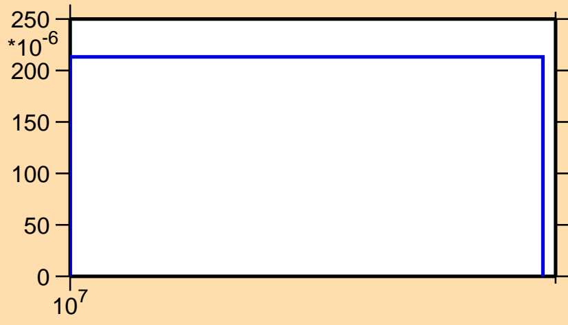
\sigma vs. E for ^{106}\text{Tc}(n,np)
