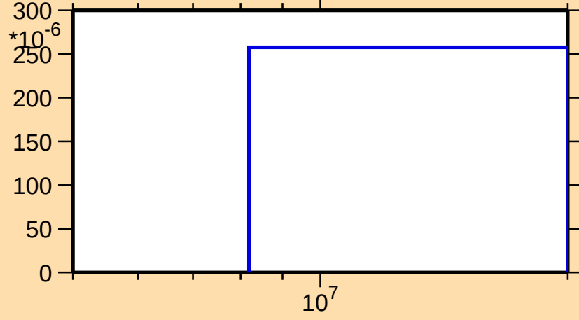
\sigma vs. E for ^{106}\text{Tc}(n,d)
