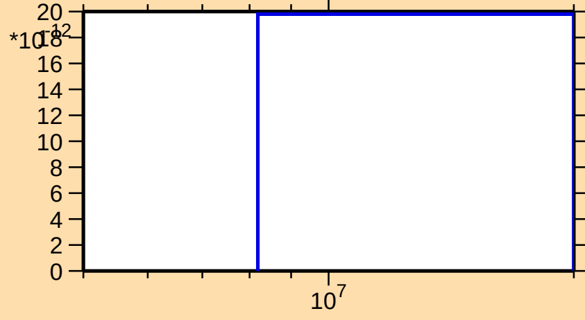
\sigma vs. E for ^{106}\text{Tc}(n,2n\alpha)
