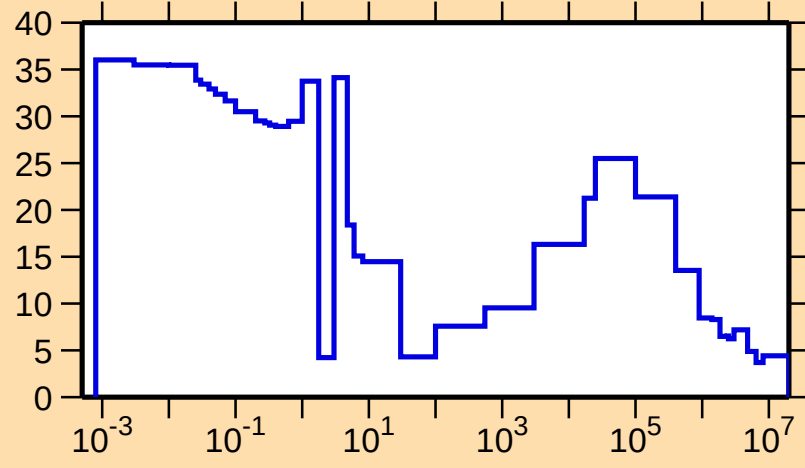
\Delta\sigma/\sigma vs. E for ^{106}\text{Tc}(n,\text{tot.})
