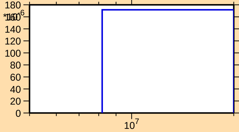
\sigma vs. E for ^{106}\text{Tc}(n,np)
