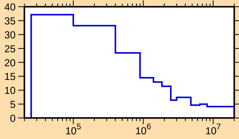
\Delta\sigma/\sigma vs. E for ^{106}\text{Tc}(n,\text{nonel.})
