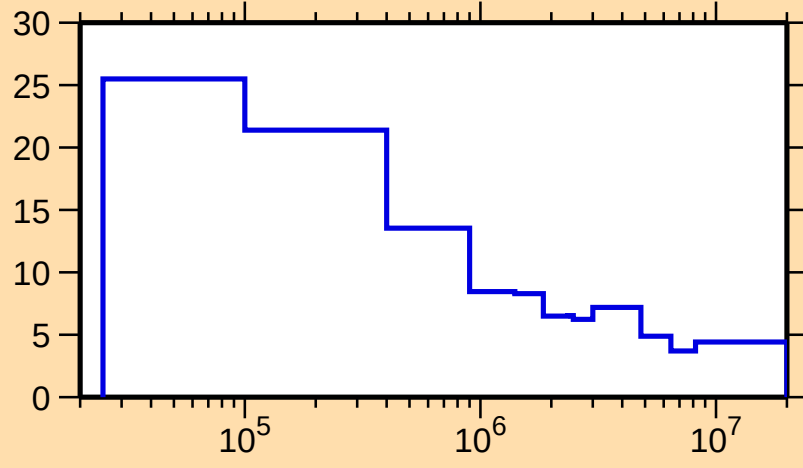
\Delta\sigma/\sigma vs. E for ^{106}\text{Tc}(n,\text{tot.})
