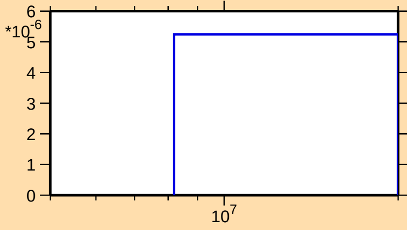
\sigma vs. E for ^{106}\text{Tc}(n,n\alpha)
