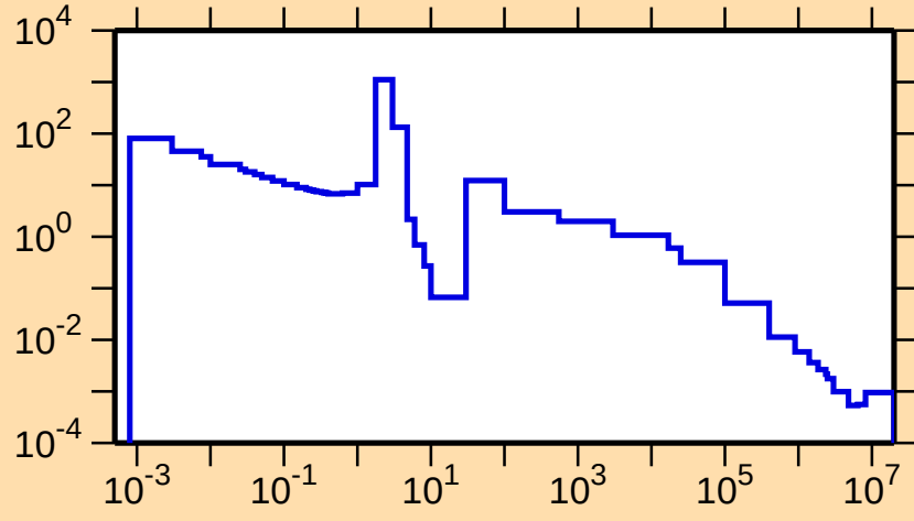
\sigma vs. E for ^{106}\text{Tc}(n,\gamma)
