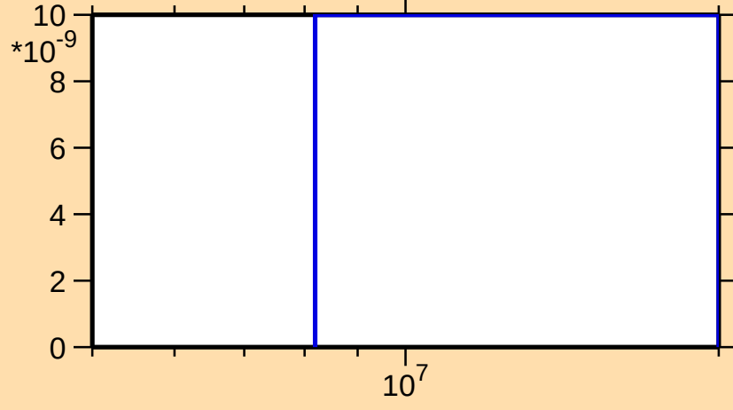
\sigma vs. E for ^{106}\text{Tc}(n,\text{nt})
