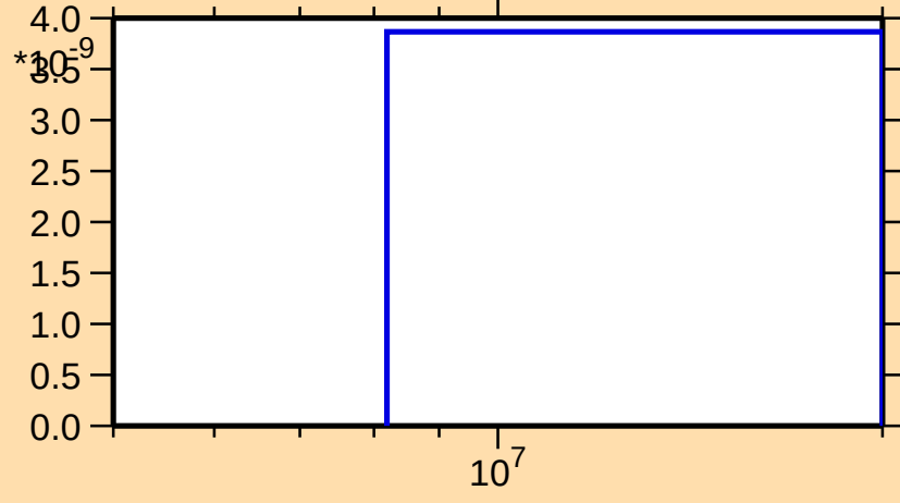
\sigma vs. E for ^{106}\text{Tc}(n,2np)
