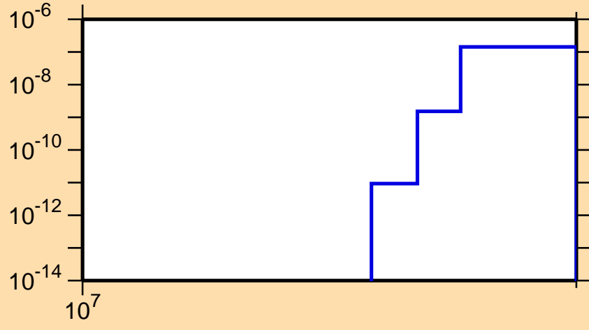
\sigma vs. E for ^{110}\text{Te}(n,\text{nd})
